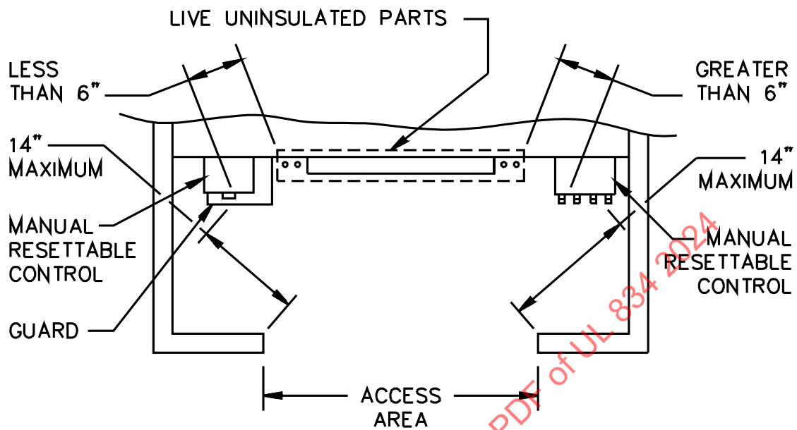
Figure 8.1 Accessibility and protection
