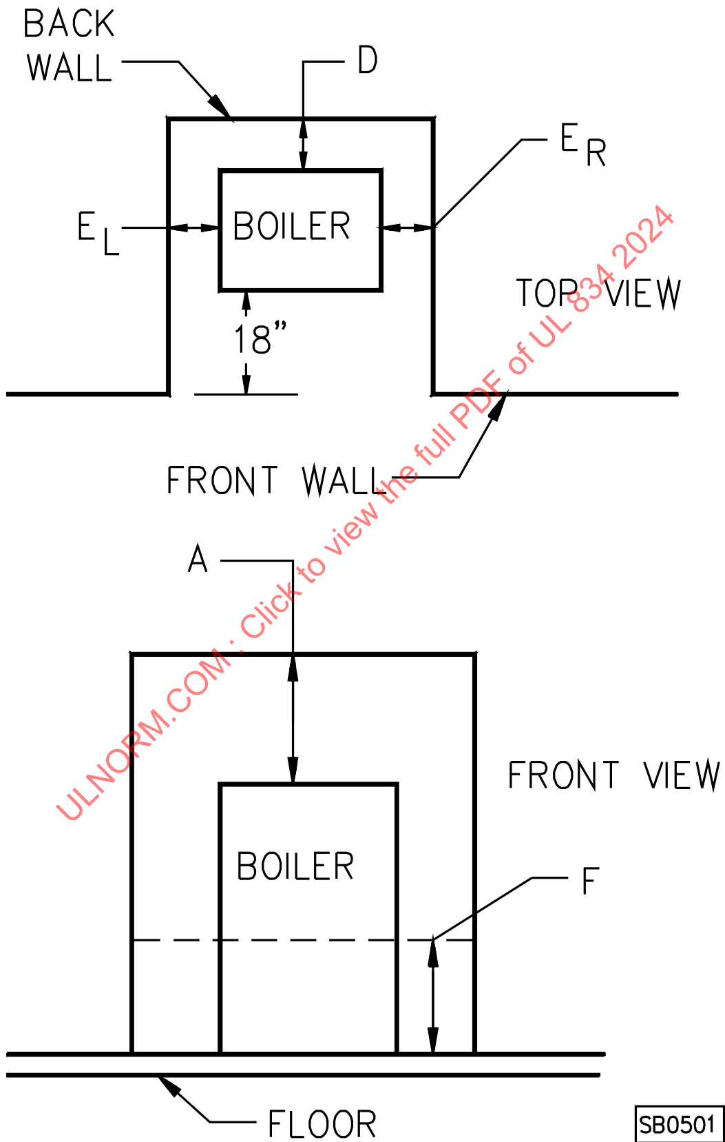
Figure 38.1 Alcove installation
