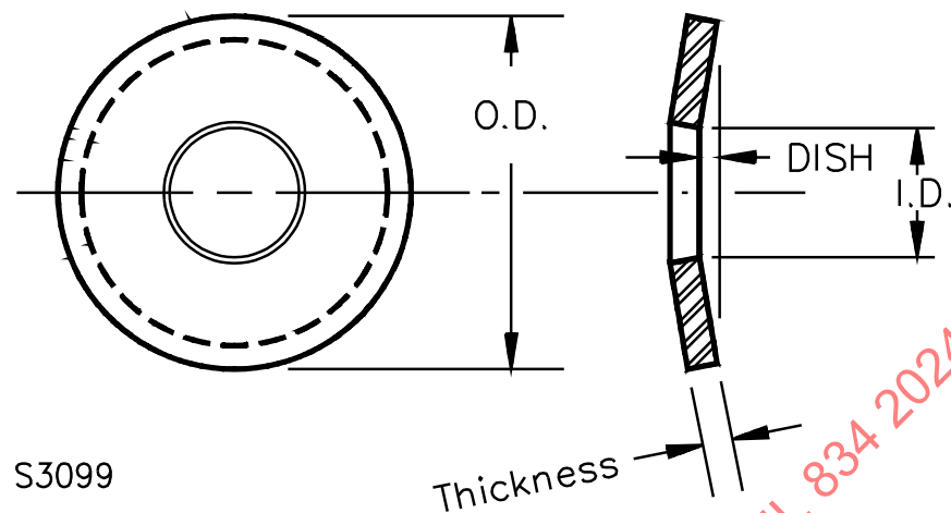
Figure 13.1 Spring washer
