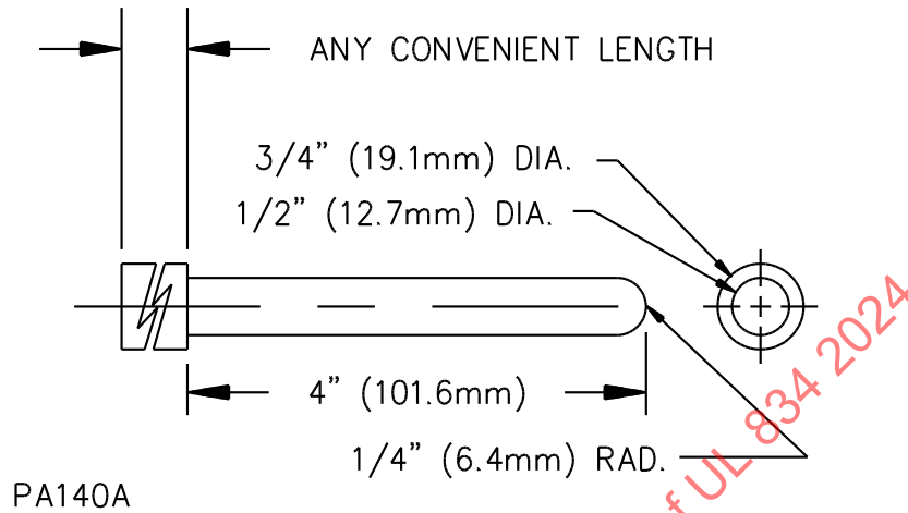
Figure 7.7 Articulate probe
