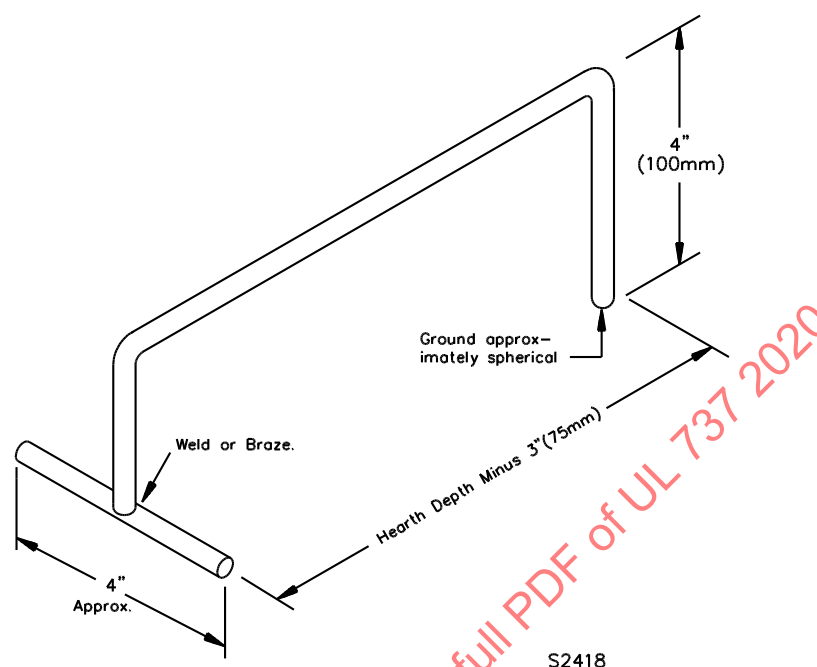
Figure 13.1 Andiron
