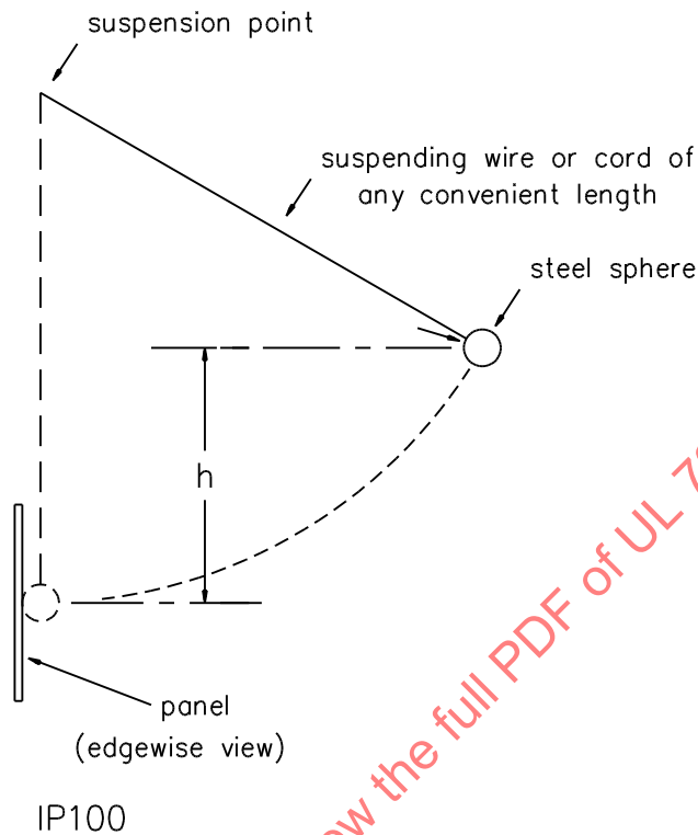
Figure 15.1 Impact test
