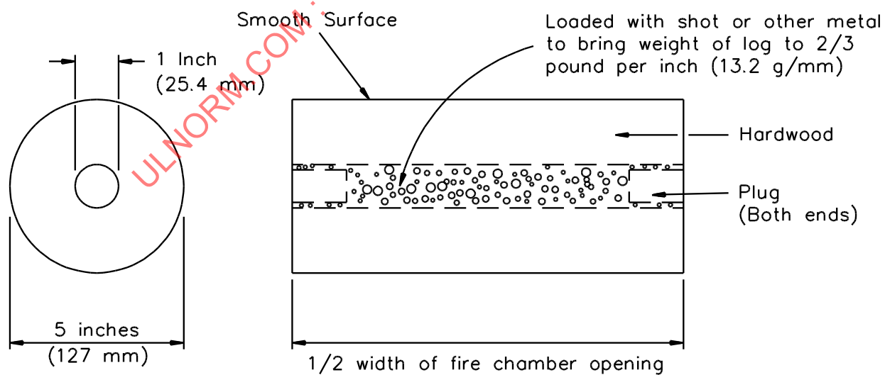
Figure 16.2 Simulated log
