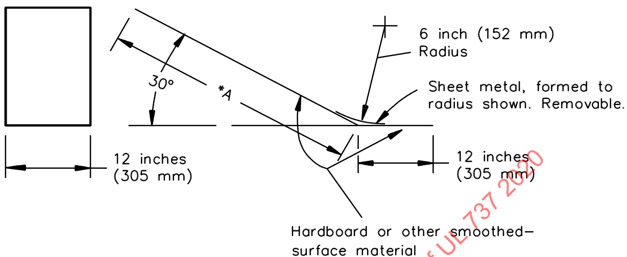
Figure 16.1 Inclined plane for strength test
