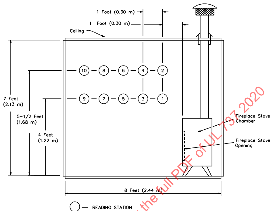
Figure 23.1 Location of carbon monoxide reading stations
