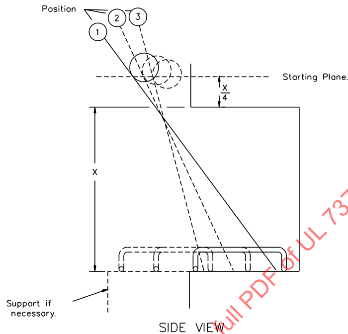
Figure 16.5 Inclined plane in position for impact test of hearth a
