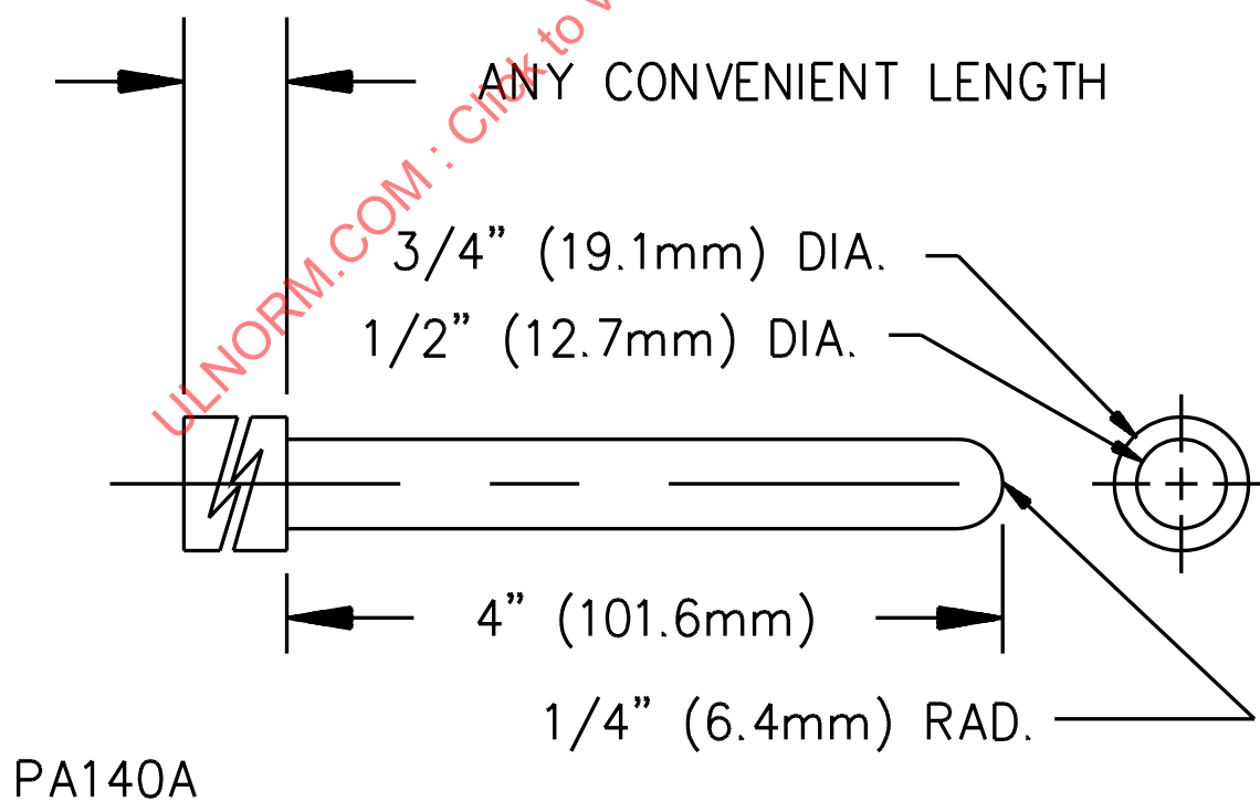
Figure 33.4 Probe for film coated wire
