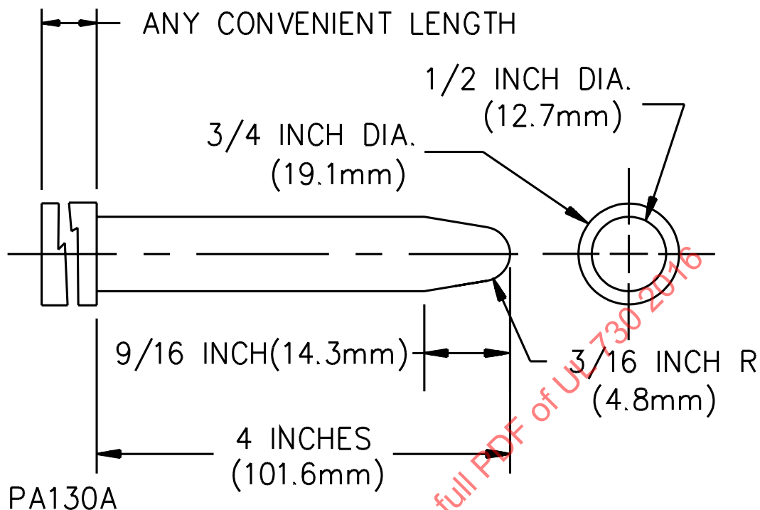
Figure 33.3 Probe for moving parts and uninsulated live parts
