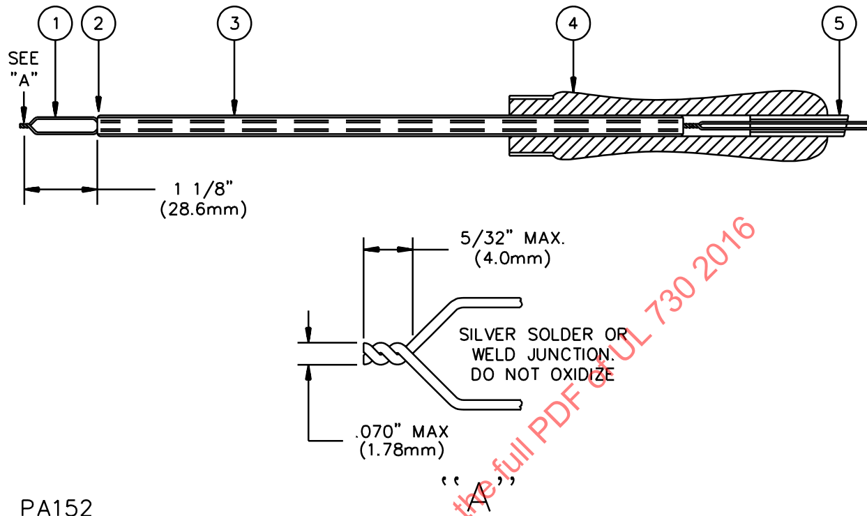
Figure 37.2 Standard thermocouple for flue-gas temperature
