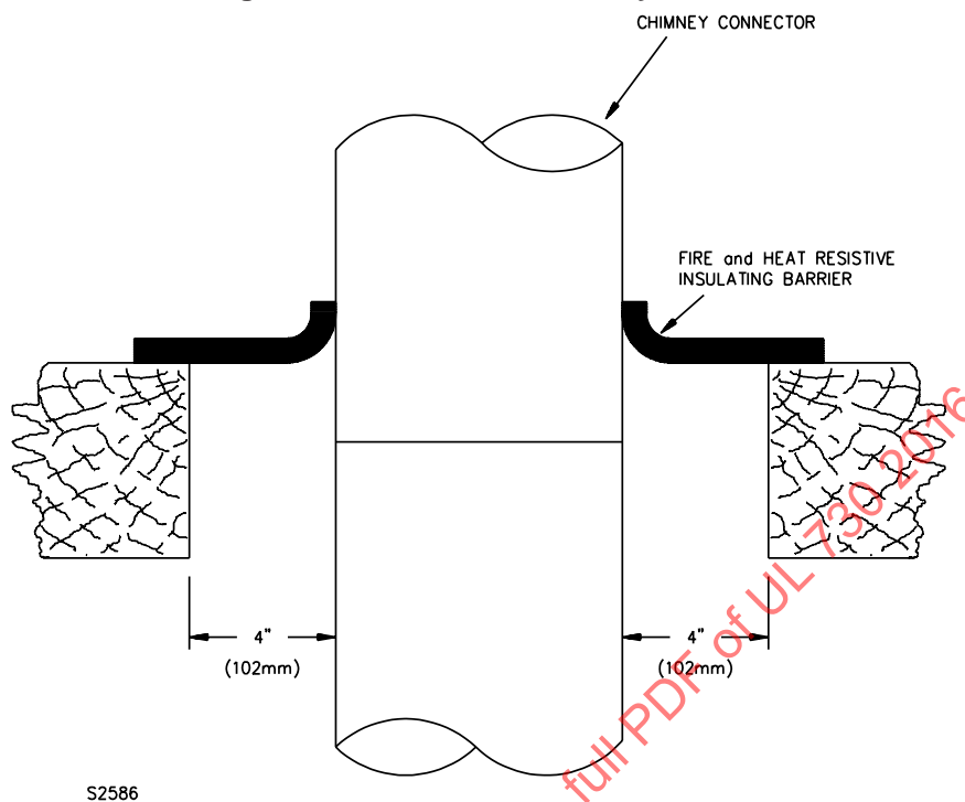
Figure 36.3 Sealing of annulus around chimney connector
