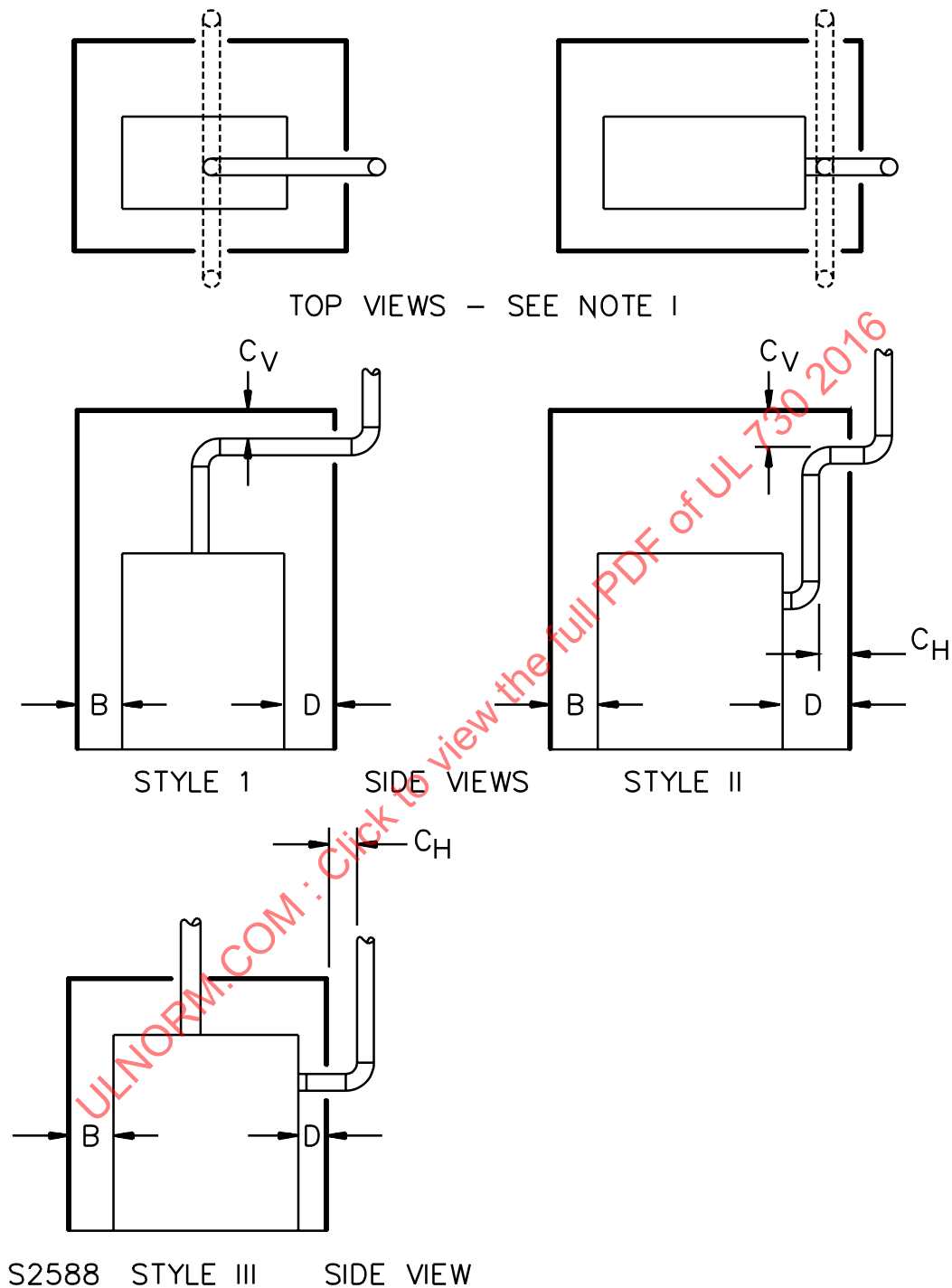
Figure 36.2 Chimney connector arrangement for alcove and closet installation
