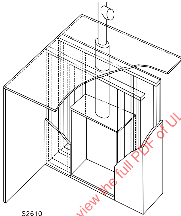
Figure 35.1 Test structure for built-in style wall furnace
