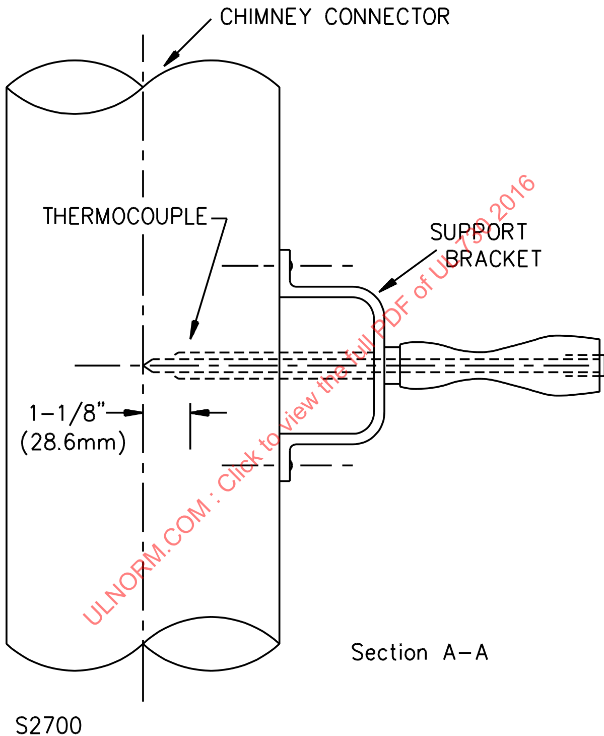
Figure 37.3 Flue gas thermocouple and support bracket
