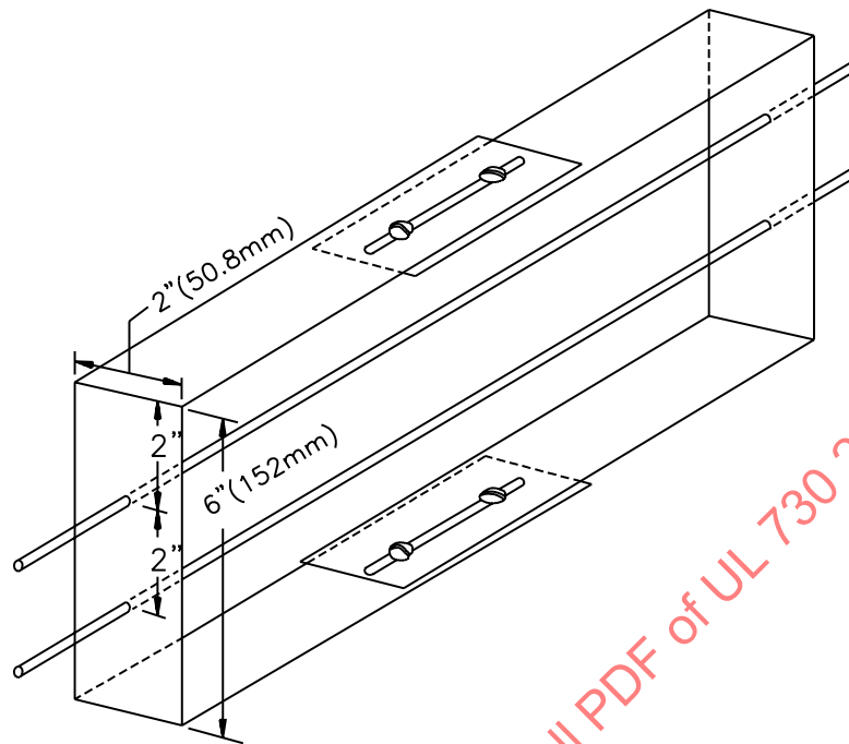
Figure 37.4 Thermocouple shield for outlet-air temperature
