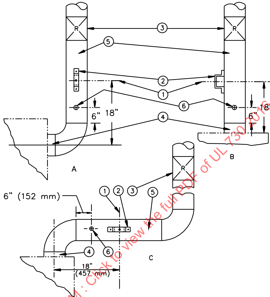
Figure 36.4 Chimney connectors – alcove and closet test
