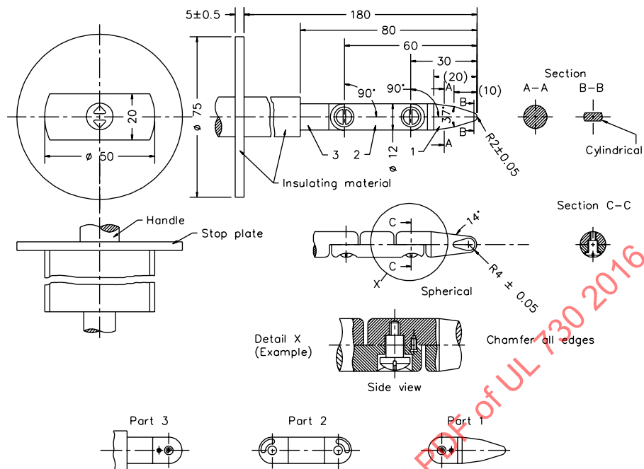
Figure 33.5 IEC articulate probe
