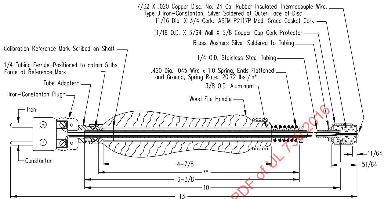
Figure 37.1 Temperature-measuring probe
