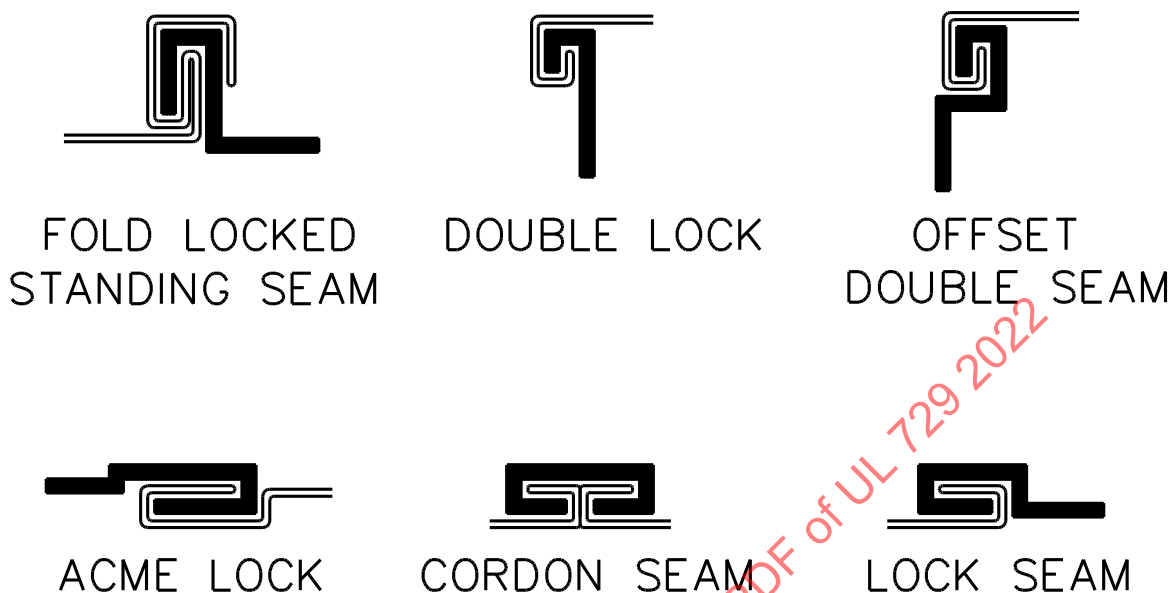
Figure 16.1 Types of acceptable lock-seams
