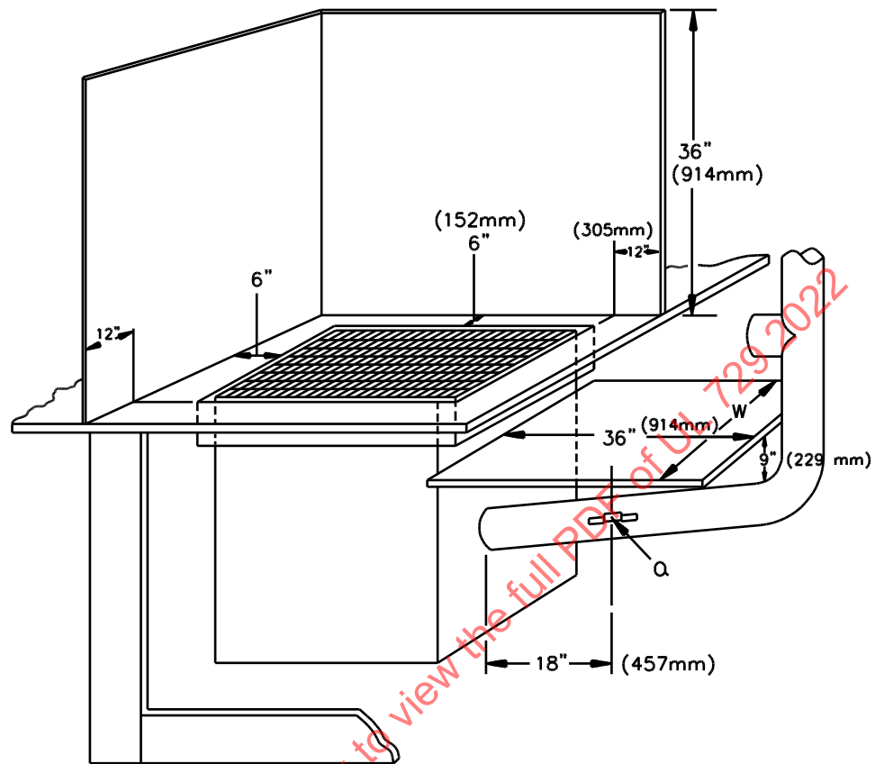
Figure 38.1 Test platform – floor register furnace
