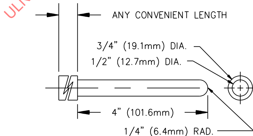
Figure 36.3 Probe for film-coated wire
