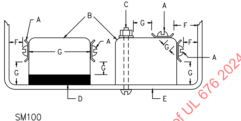
Figure 23.1 Spacings at wiring devices
