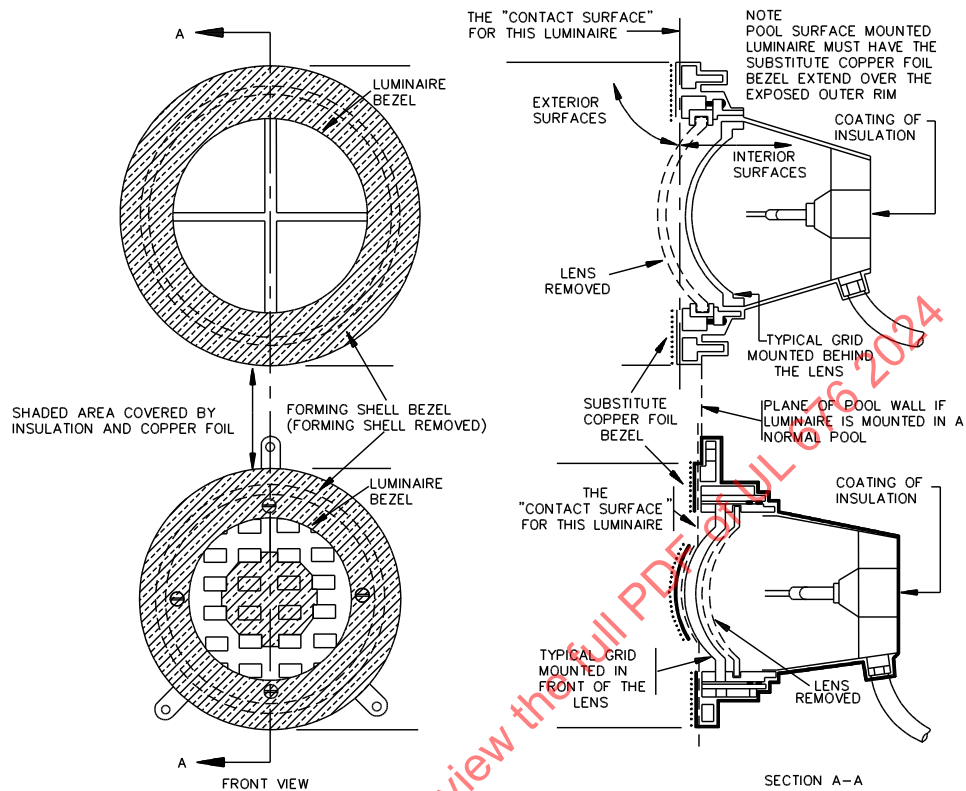
Figure 41.1 Test modified luminaire
