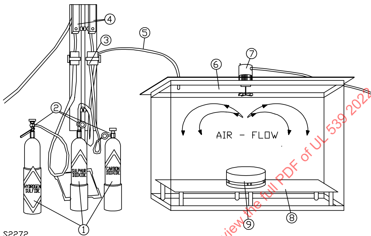
Figure 35.1 Corrosion Test Setup
