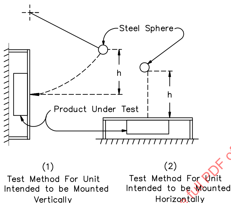
Figure 46.1 Jarring Test
