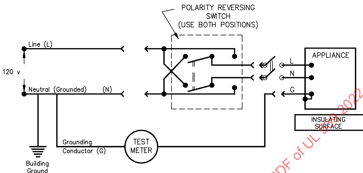
Figure 58.1 Leakage Current Measurement Circuit
