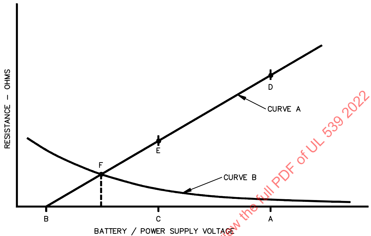
Figure 51.2 Trouble Level Determination
