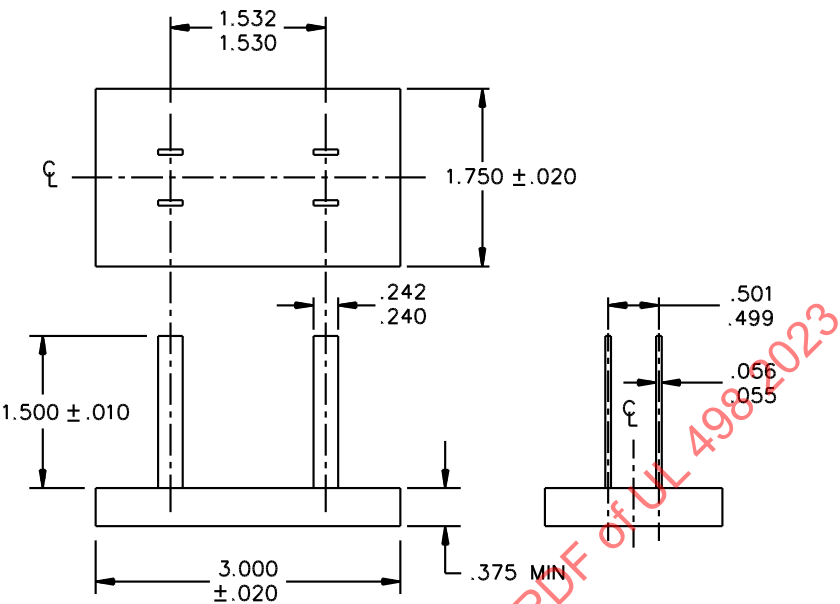
Figure 124.3 Pushout tool
