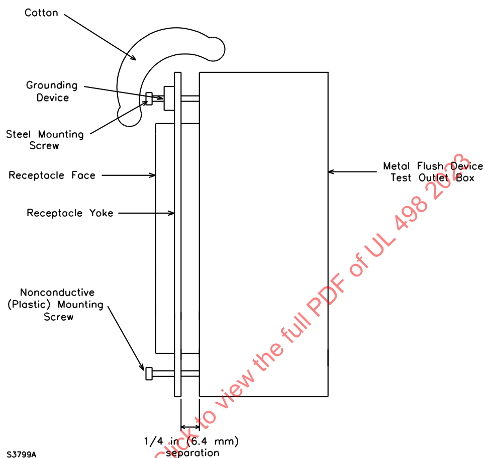
Figure 130.1 Fault current assembly
