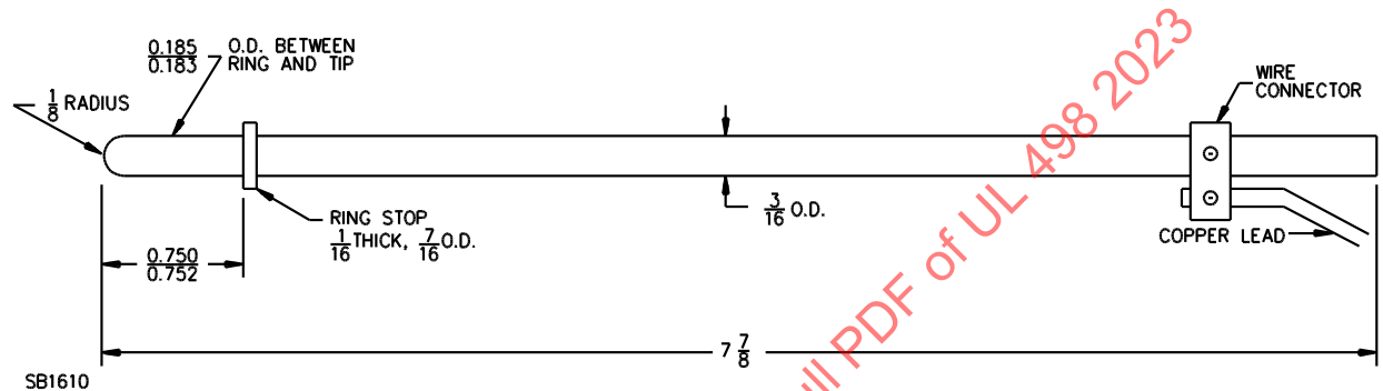
Figure 125.2 Test pin B
