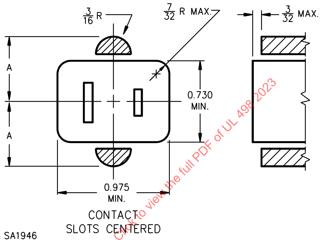
Figure 23.3 Minimum outlet face dimensions
