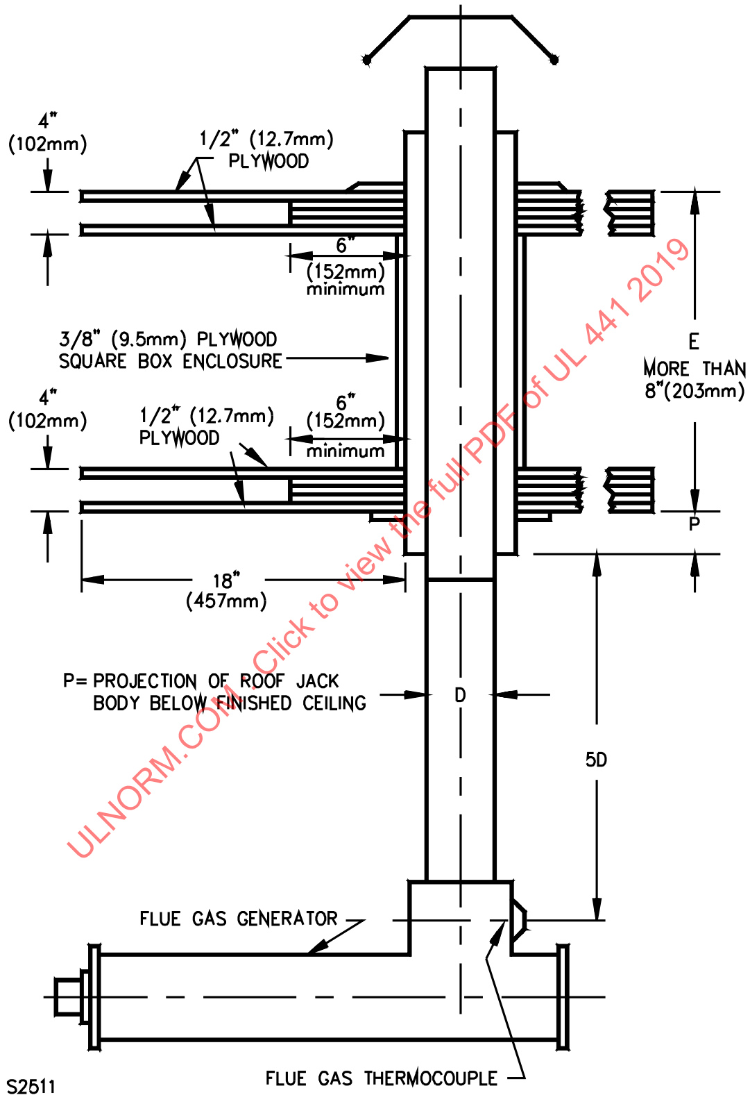
Figure 19.8 Test structure – Form V – for Type B gas vent roof jacks, roof and ceiling
