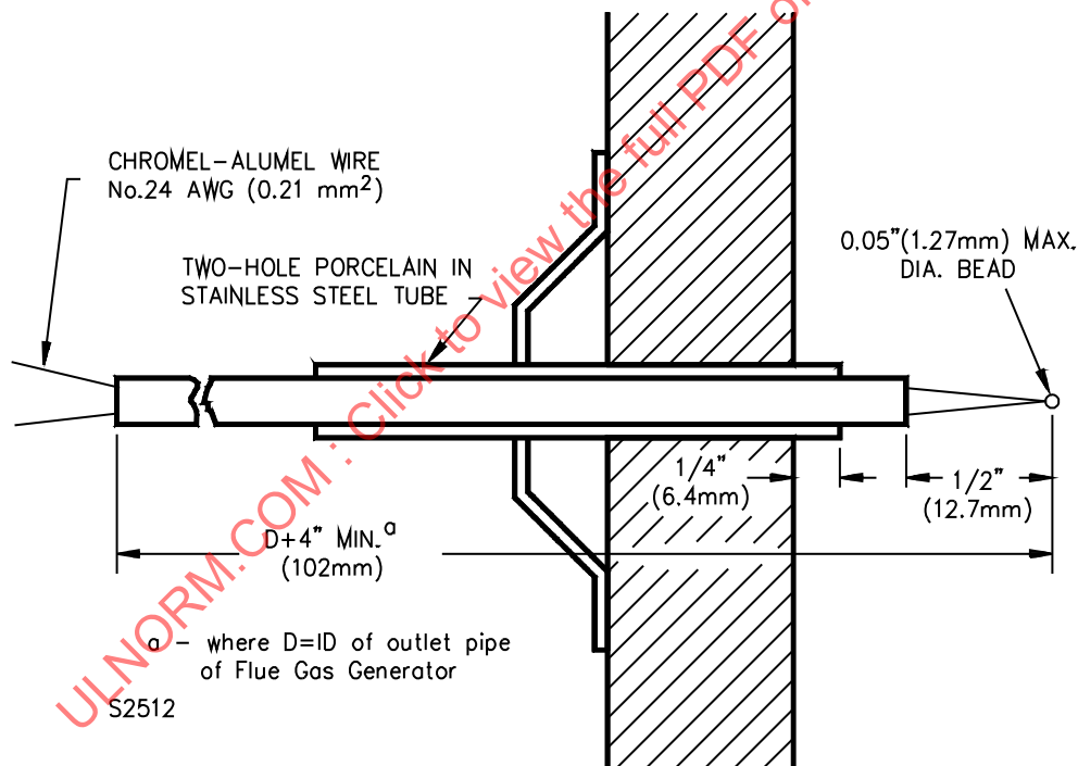
Figure 20.1 Flue-gas thermocouple and support bracket
