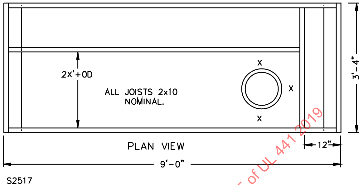
Figure 19.3 Test structure details – Form I – for large diameter Type B vents
