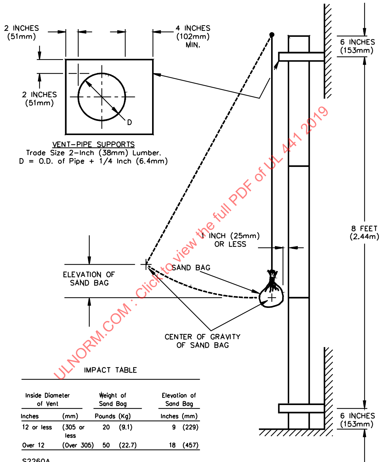
Figure 25.1 Strength test
