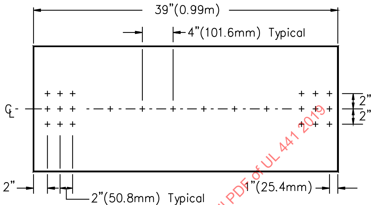
Figure 20.4 Thermocouple pattern for test structure – Forms III and VI
