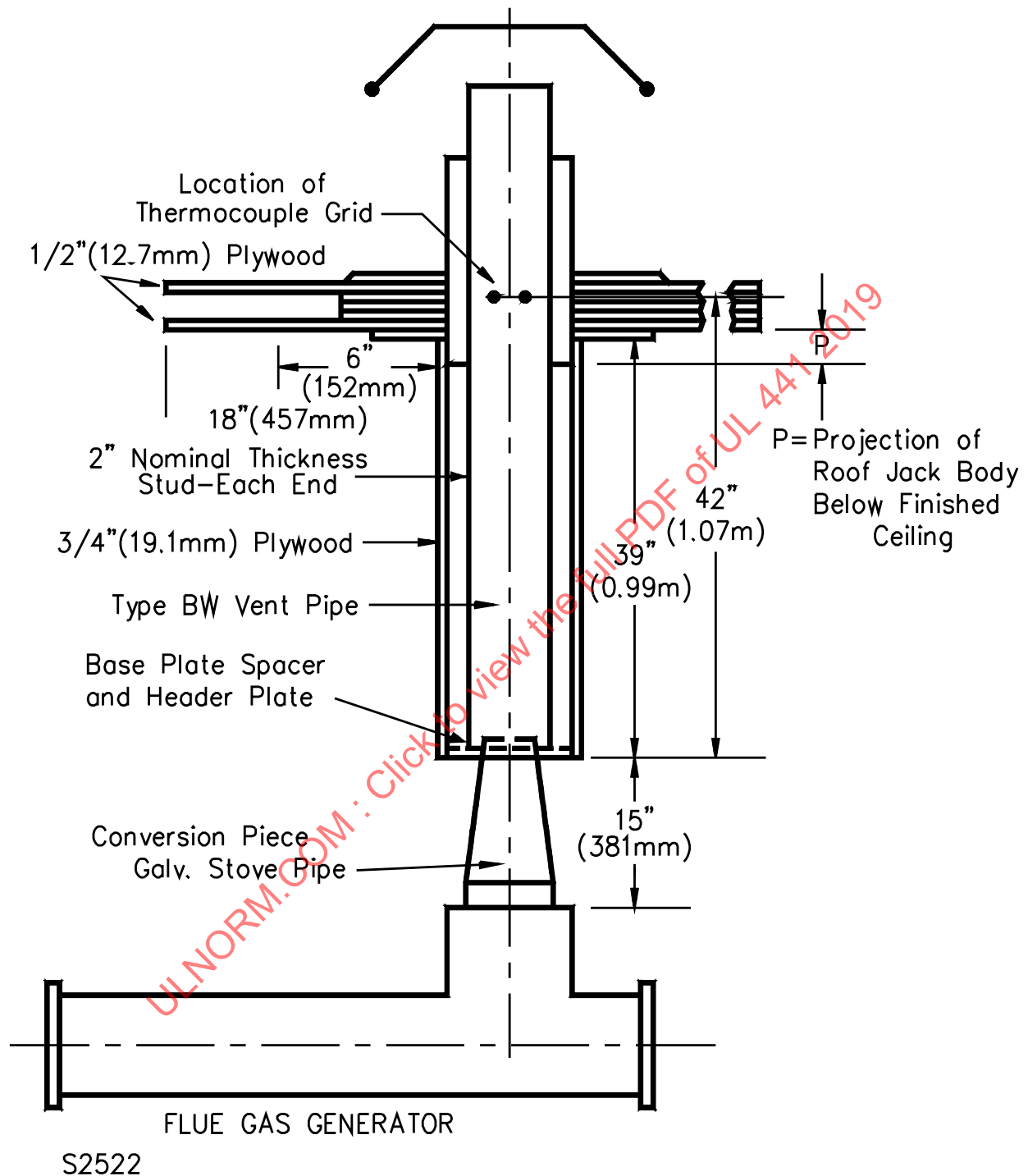
Figure 19.9 Test structure – Form VI – for Type BW gas vent roof jacks
