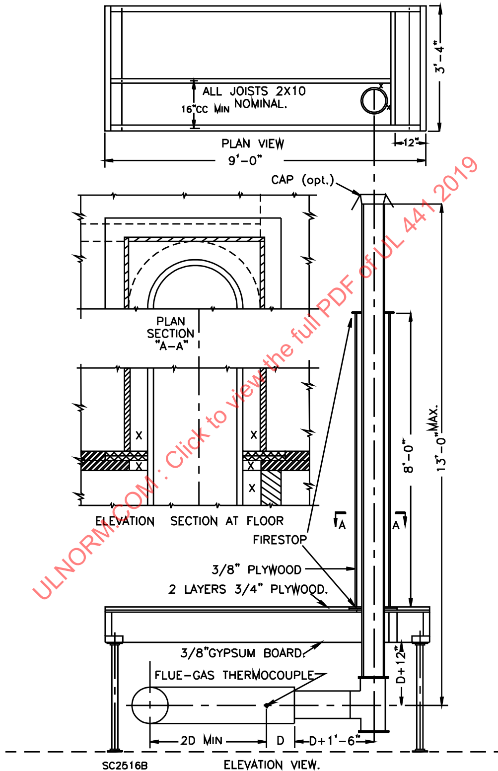
Figure 19.1 Test structure – Form I – for Type B vents Enclosure shown at a specified clearance denoted by "X"
