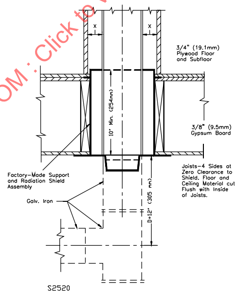
Figure 19.4 Test structure details – Form I – for support assembly with radiation shield
