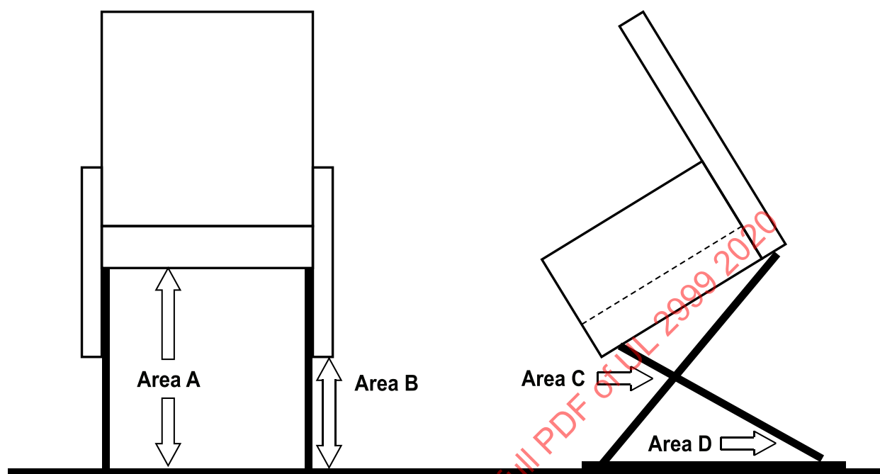
Figure 53.2 Examples of entrapment areas
