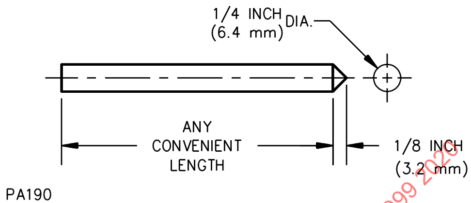
Figure 13.4 Accessibility probe
