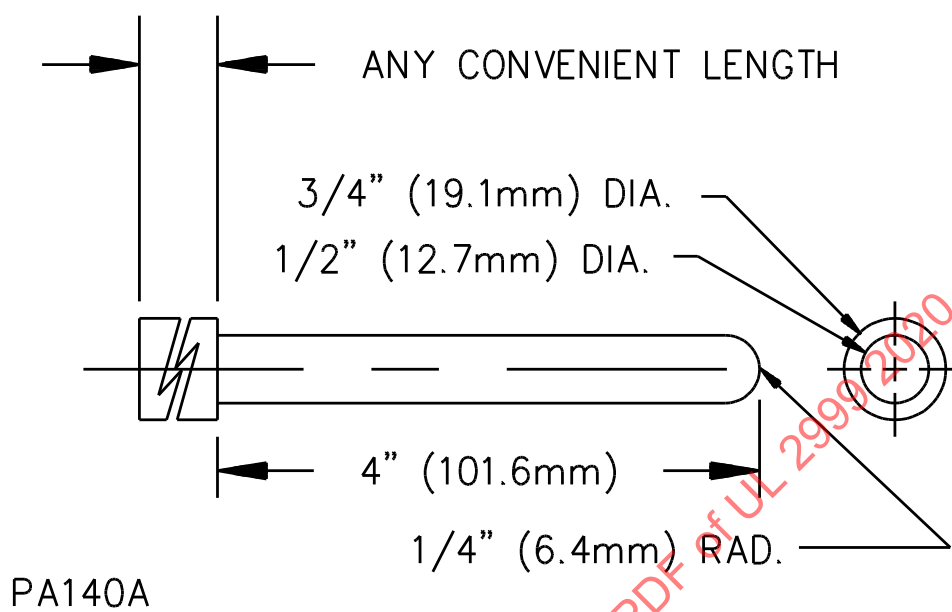
Figure 13.3 Straight probe
