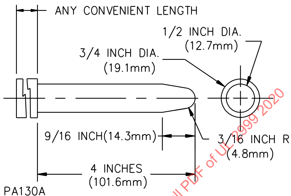
Figure 13.2 Straight probe
