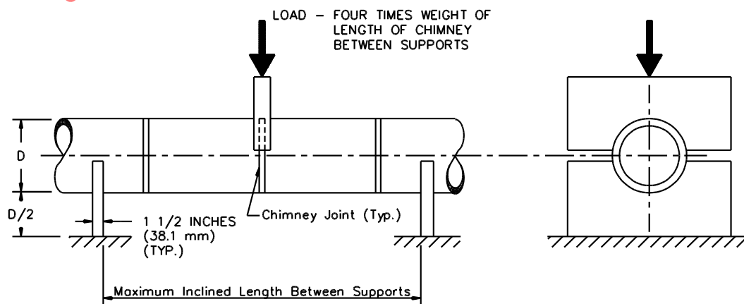
Figure 21.3 Chimney joint load test
