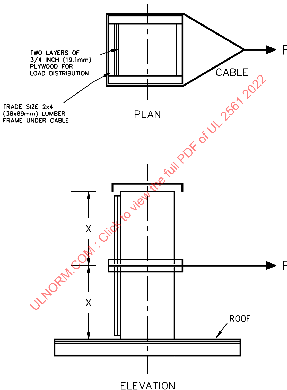
Figure 22.1 Wind load test on roof assembly
