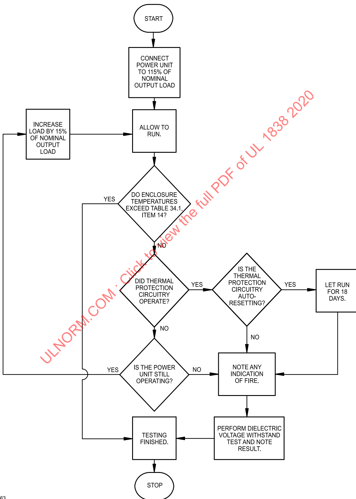
Figure 29.1 Overload test flow chart
