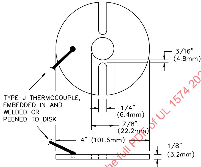
Figure 54.1 Temperature probe for supply wire temperatures
