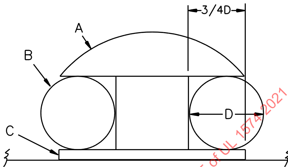
Figure 24.1 Terminal-conductor relationship
