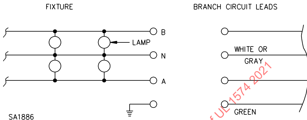
Figure 23.2 120/240-volt system
