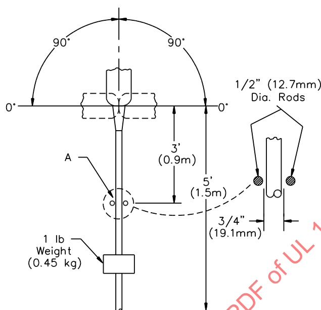
Figure 39.1 Cord flexing
