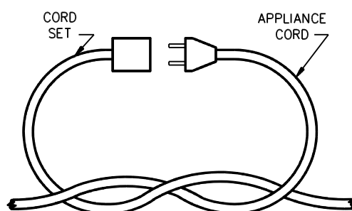
(A) TIE CORD AS SHOWN
