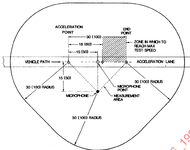
FIG. 1—MINIMUM UNIDIRECTIONAL TEST SITE (SEE PARAGRAPH 3.1)
