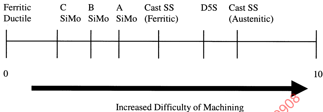
FIGURE 2—RELATIVE MACHINABILITY IN VARIOUS MATERIALS
