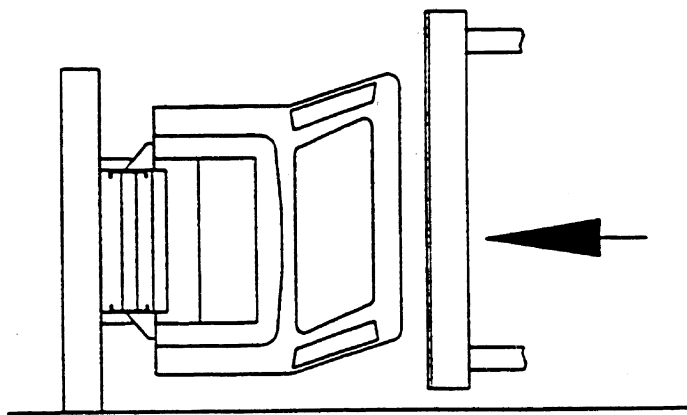
FIGURE 5—QUASI-STATIC ROOF LOAD CONFIGURATION
