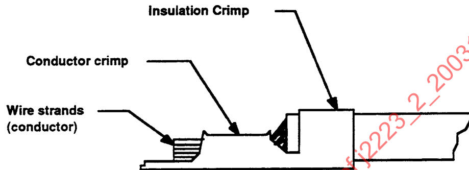
FIGURE 6—CONDUCTOR AND INSULATION CRIMP
