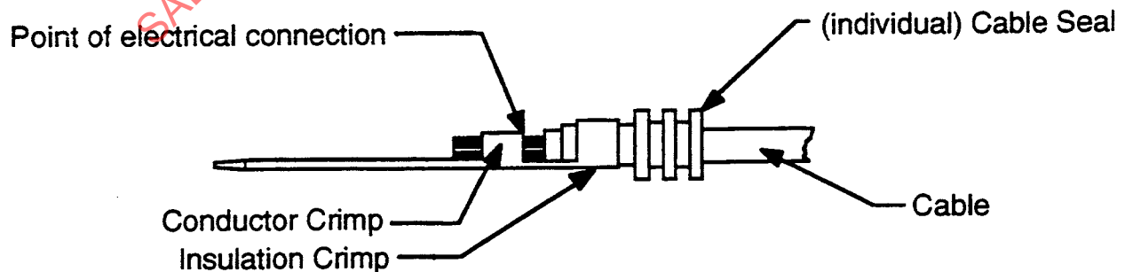
FIGURE 1—MALE TERMINAL
