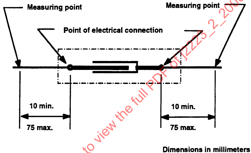
FIGURE 7—CONNECTION RESISTANCE—CABLE-TO-CABLE CONNECTION
