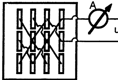
FIGURE 10—LEAKAGE CURRENT MEASUREMENTS BETWEEN ADJACENT CONTACTS (EXAMPLE)
