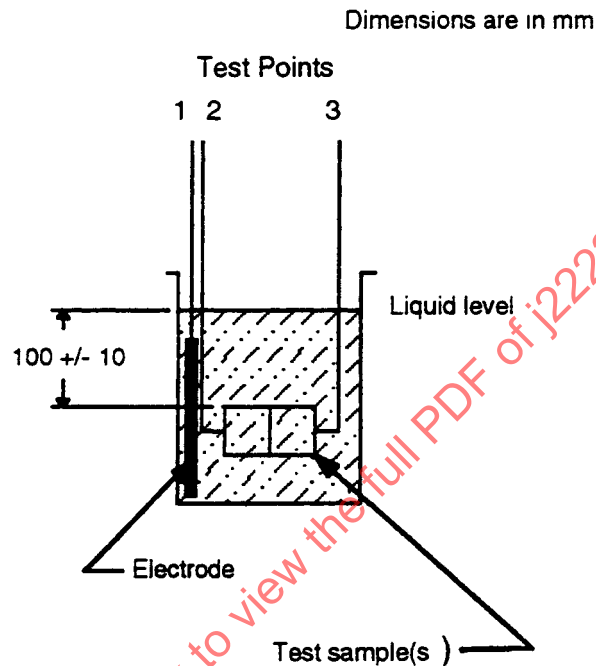
FIGURE 9—WATER TIGHTNESS TEST
