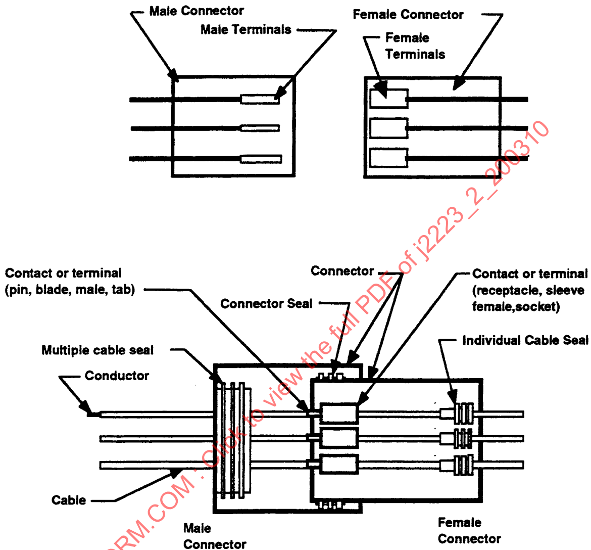
FIGURE 4—MULTIPOLE CONNECTORS/CONNECTIONS
