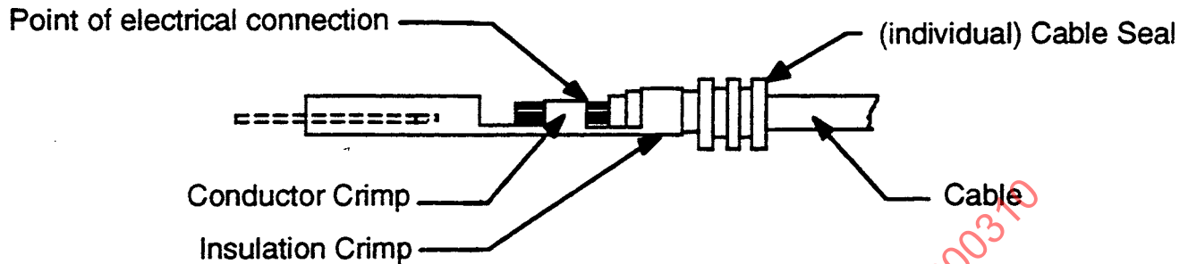
FIGURE 2—FEMALE TERMINAL
