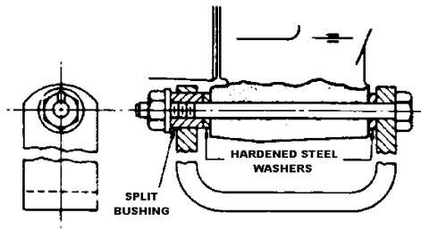
FIGURE 4—TYPICAL INSTALLATION OF SPLIT BUSHING IN BRACKET FOR SPOOL MOUNTING
