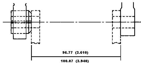
FIGURE 3—TYPICAL INSTALLATION OF SPLIT BUSHING IN HINGE MOUNTING LUG
