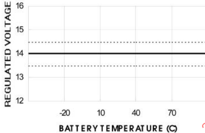
FIGURE 5—FLAT COMPENSATION CURVE
