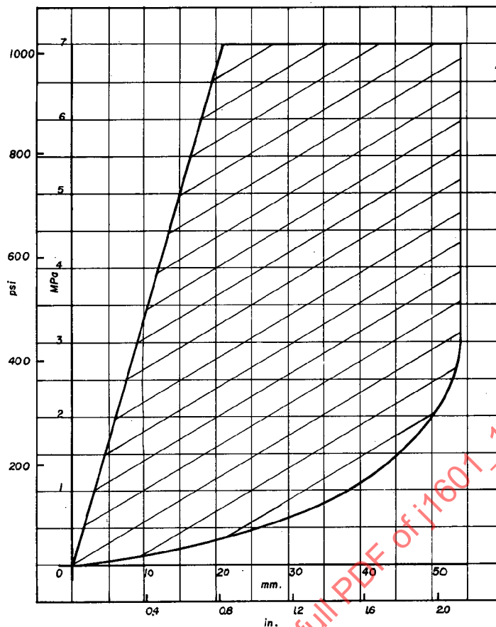
FIG. 2 - TYPICAL WHEEL CYLINDER CUP STROKE VERSUS PRESSURE 12.7 TO 50.8 MM (1/2 TO 2 IN) DIAMETER
