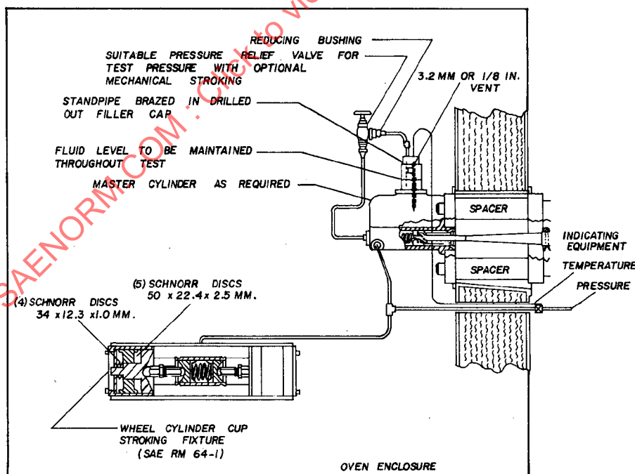
FIG. 1 - RECOMMENDED WHEEL AND MASTER TEST CYLINDER APPARATUS
