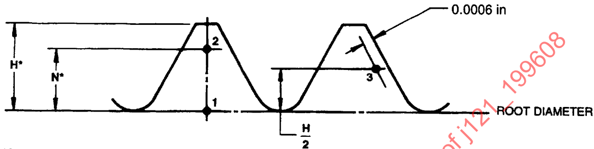
(R) FIGURE 2—POSITIONS FOR DETERMINING HARDNESS
