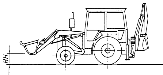
FIGURE A2—BACKHOE-LOADER
