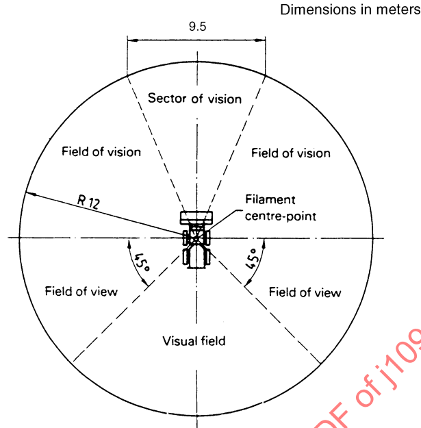
FIGURE 2—DEFINITION OF VISIBILITY TEST AREAS (SEE SECTION 3)
