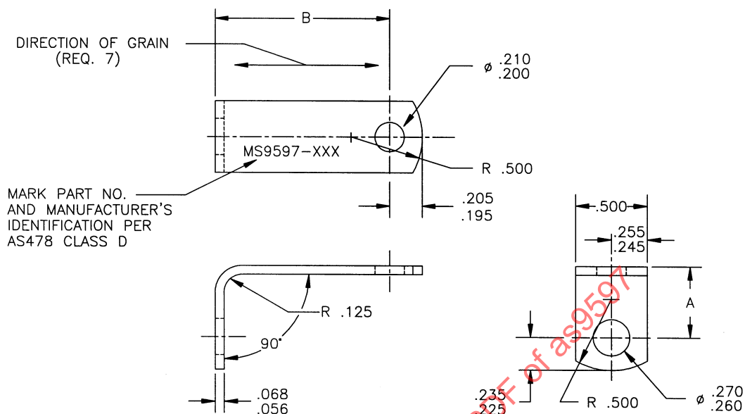
FIGURE 1 - ANGLE BRACKET
