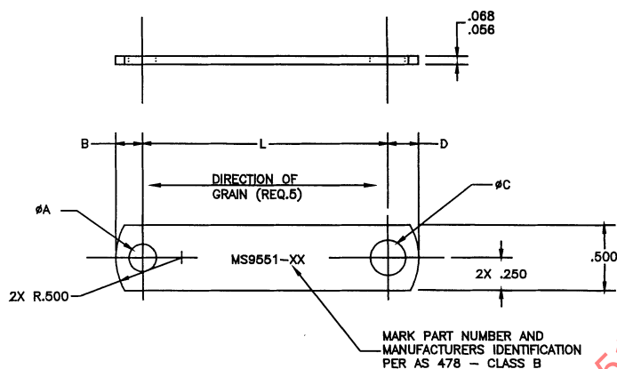
FIGURE 1. BRACKET
