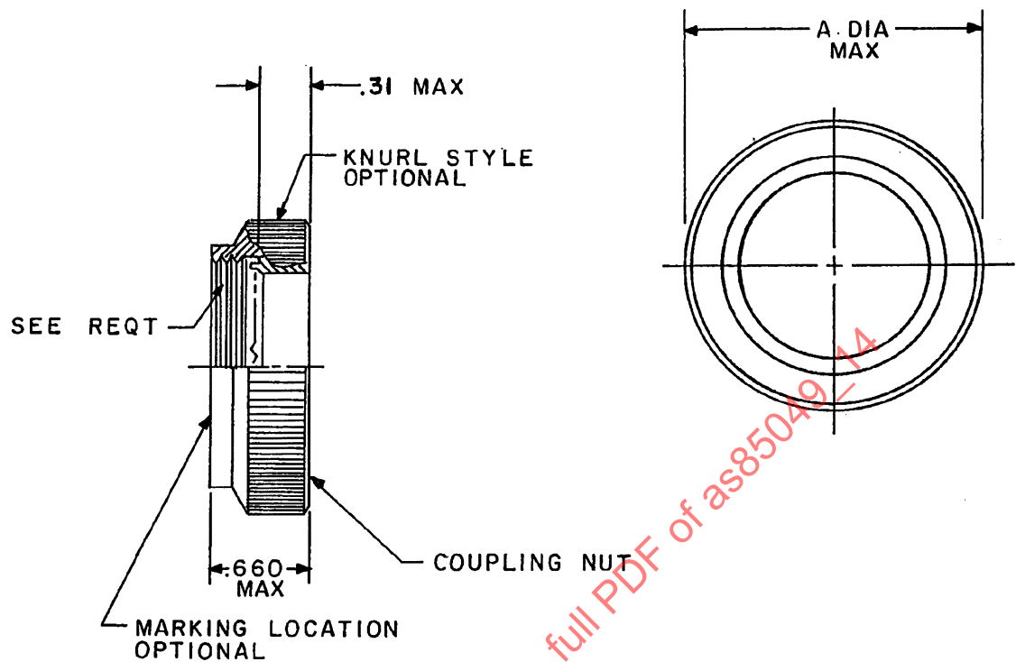
FIGURE 1. DIMENSIONS AND CONFIGURATIONS.
