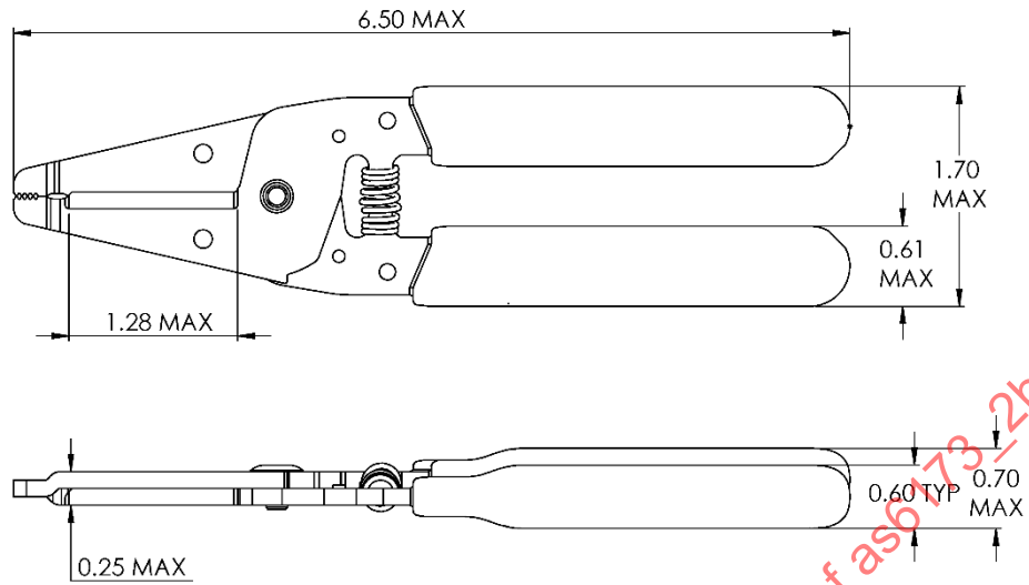
FIGURE 1 - BASIC WIRE CUTTER TOOL
