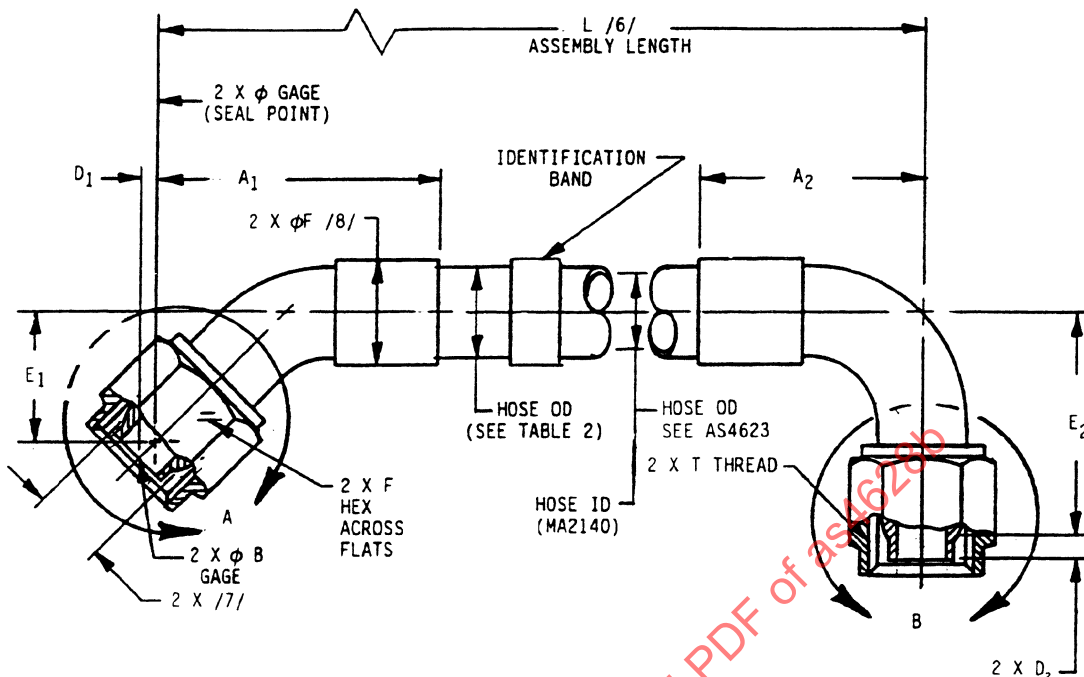
FIGURE 1 - HOSE ASSEMBLY, 45° ELBOW TO 90° ELBOW
