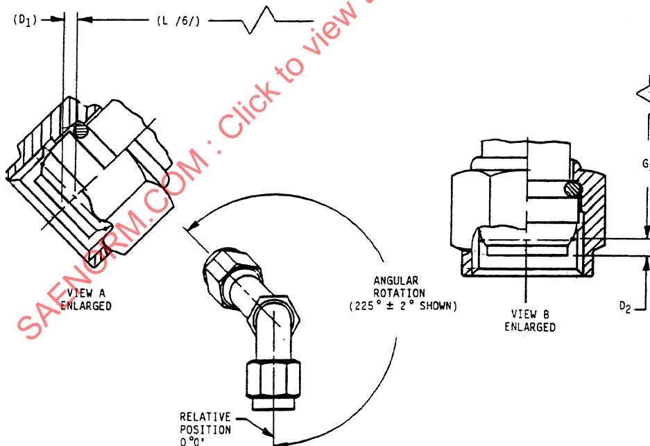
FIGURE 2 - FITTING ORIENTATION /19/
