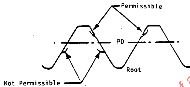
FIGURE 7 - Laps Extending Towards Crest, Rolled Thread
