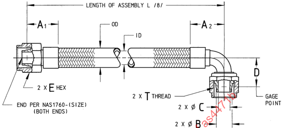
FIGURE 1 - HOSE ASSEMBLY
