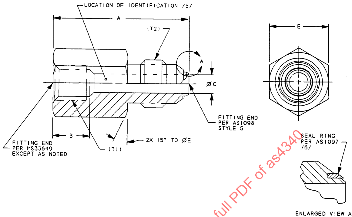
FIGURE 1 - BUSHING, SCREW THREAD REDUCER
