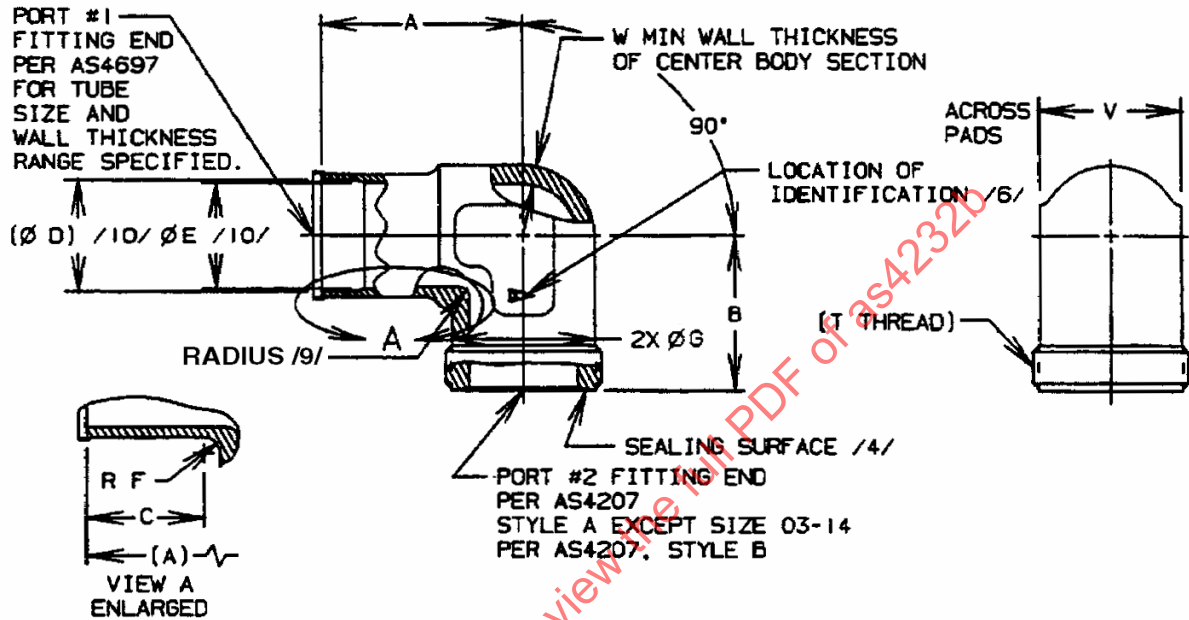
FIGURE 1 - FITTING, ELBOW, 90°
