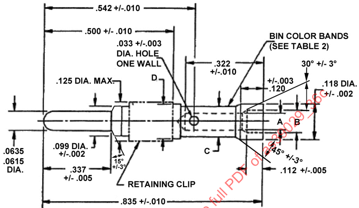
FIGURE 1 - AS39029/36 PIN CONTACT
