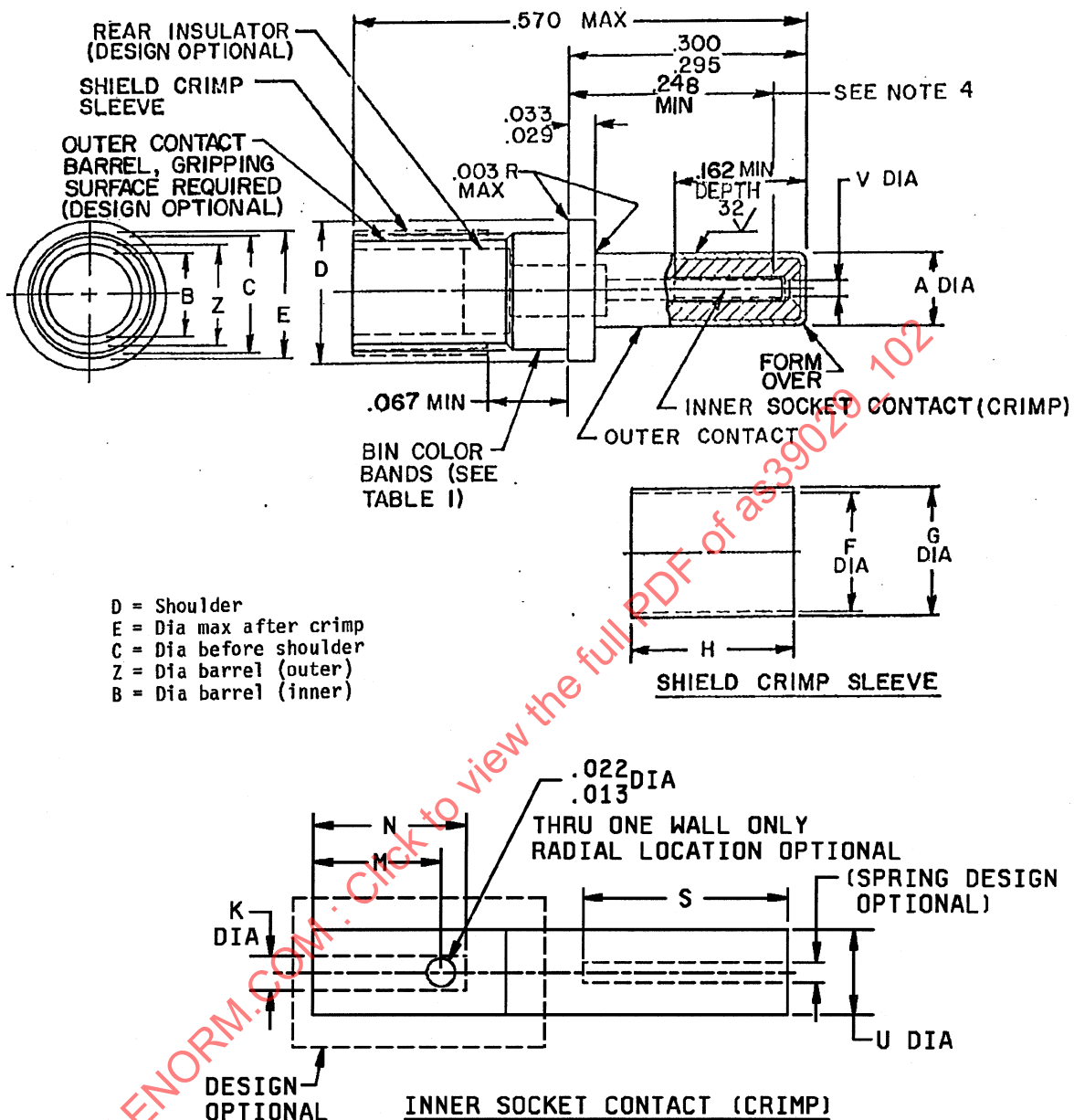
FIGURE 1. PIN CONTACTS.
