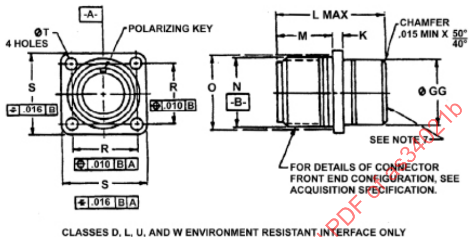
FIGURE 1 – CONNECTOR CONFIGURATION AND DIMENSIONS
