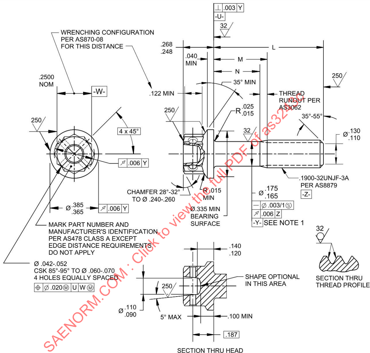
FIGURE 1 - BOLT
