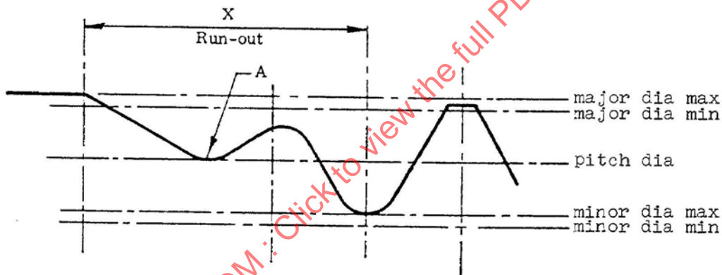
FIGURE 2A. Full Shank Fasteners
