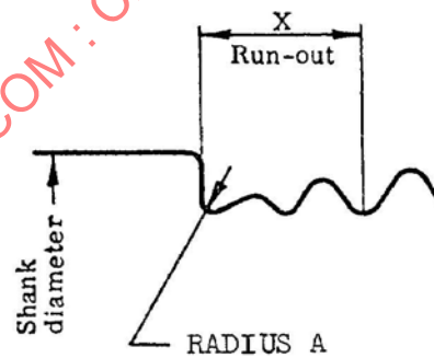
FIGURE 8D - Shoulder Bolt
