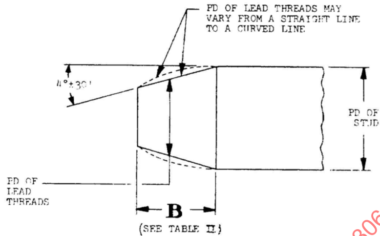
FIGURE 5 For Illustrative Purposes Only
