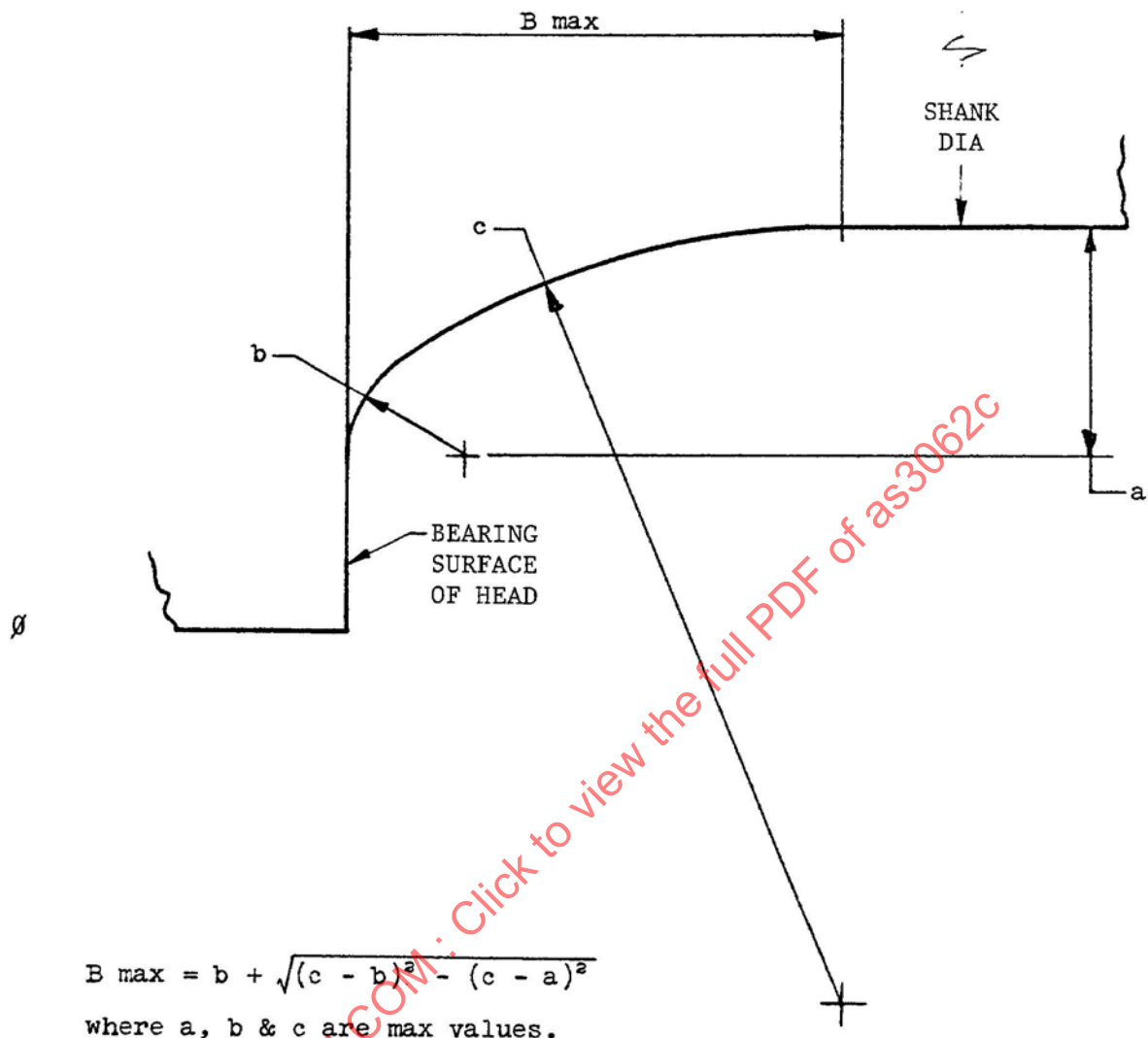
FIGURE 9 - Max Length of Head-to-Shank Compound Fillet, B Max
