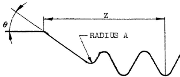
FIGURE 10 - Oversize Shank Bolts
