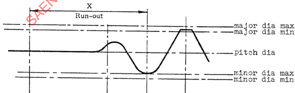
FIGURE 2B. Pitch Diameter Shank Fasteners
