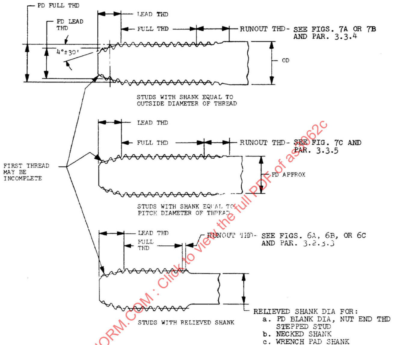
FIGURE 4. Stud End For Illustrative Purposes Only
