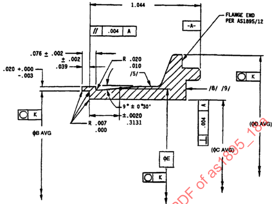
FIGURE 1 - TYPICAL VIEW
