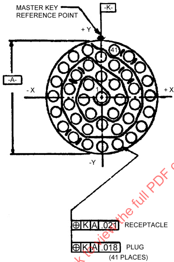
FIGURE 1 - INSERT CONFIGURATION
