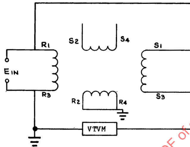
A Approximate Electrical Zero - Rotor excited resolvers.
