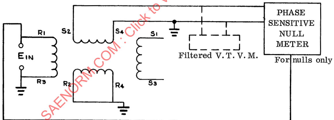
B Electrical Zero Rotor excited Resolvers
