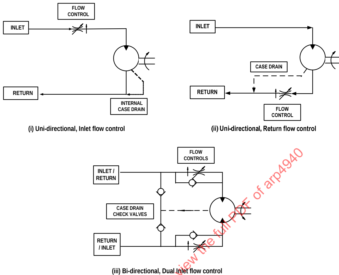
FIGURE 7 - FLOW CONTROL CONCEPTS FOR FIXED DISPLACEMENT MOTORS
