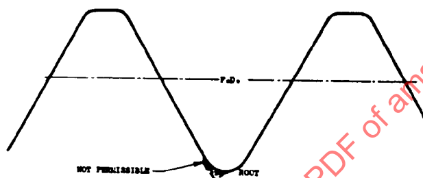
FIGURE 3 ROLLED THREAD
