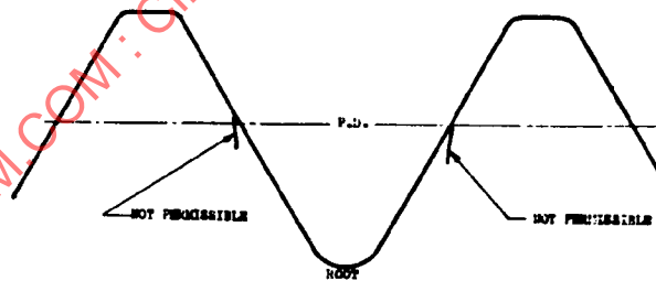
FIGURE 4 ROLLED THREAD
