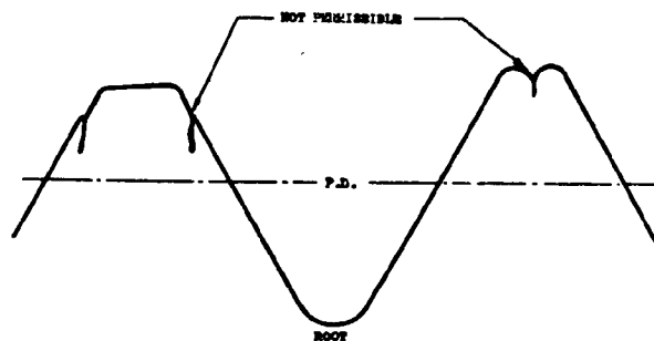
FIGURE 5 ROLLED THREAD
