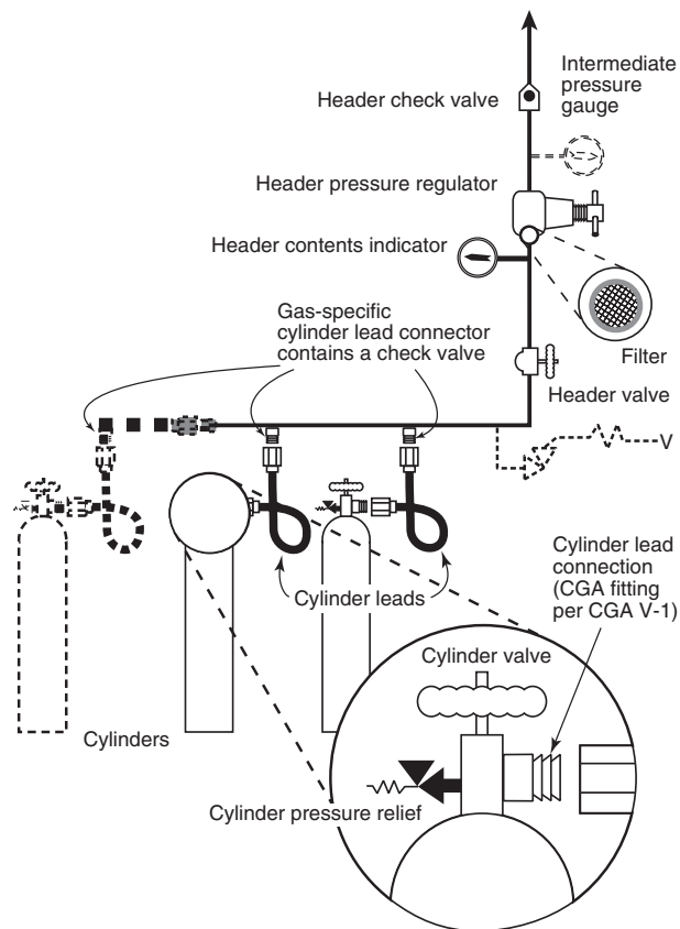
FIGURE A.5.1.3.4.9(a) Header for Gas in Cylinders.
