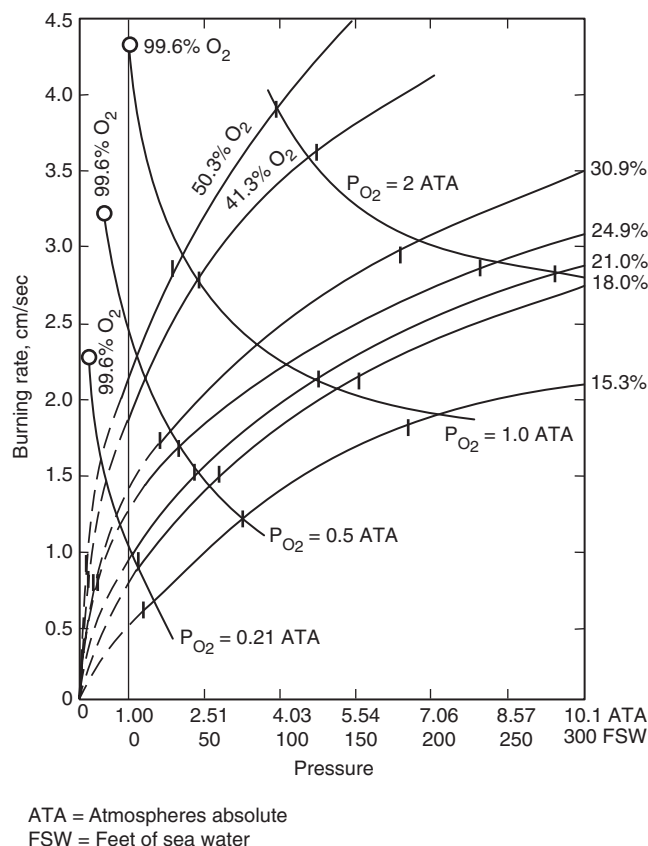
FIGURE A.3.3.14.3 Burning Rates of Filter Paper Strips at an Angle of 45 Degrees in N_2 - O_2 Mixtures. (Adapted from Figure 4 of "Technical Memorandum UCRI-720, Chamber Fire Safety.")
