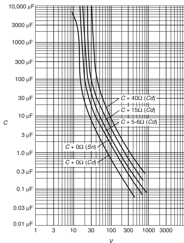
FIGURE 10.2.9.3(f) Capacitance Circuits Minimum Ignition Voltages. The curves correspond to values of current-limiting resistance as indicated. The curve marked Sn is applicable only where cadmium, zinc, or magnesium can be excluded.
