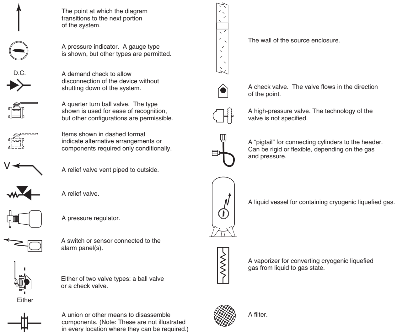
FIGURE A.5.1.3 Legend for Typical Level 1 Source Drawings.
