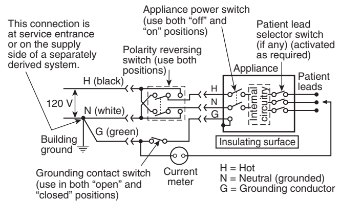
FIGURE 10.2.13.5.2.3 Test Circuit for Measuring Leakage Current Between Patient Leads and Ground (Isolated).
