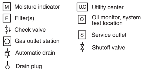
FIGURE A.5.3.3.5 Level 3 Gas-Powered Devices Supply System.
