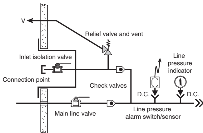
FIGURE A.5.1.3.4.14 Emergency Oxygen Supply Connection.
