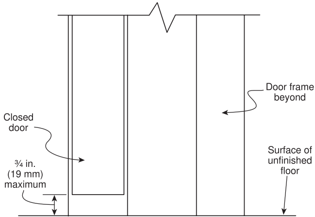
▲ FIGURE A.4.8.4.2(a) Clearance Between Bottom of Door and Unfinished Floor.
