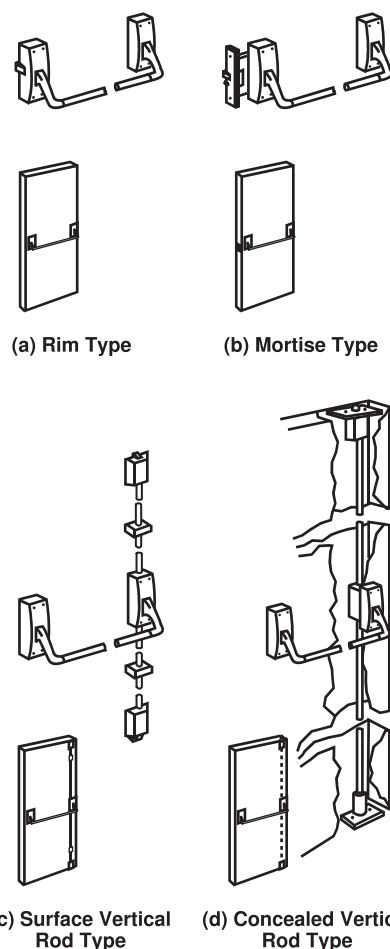
FIGURE A.4.6.3.1(e) Types of Fire Exit Hardware.
