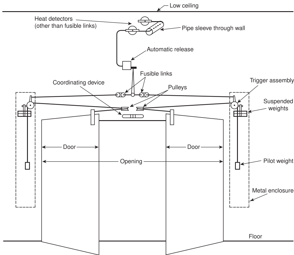
N FIGURE A.7.1(d) Closing Devices for Doors Swinging in Pairs.
