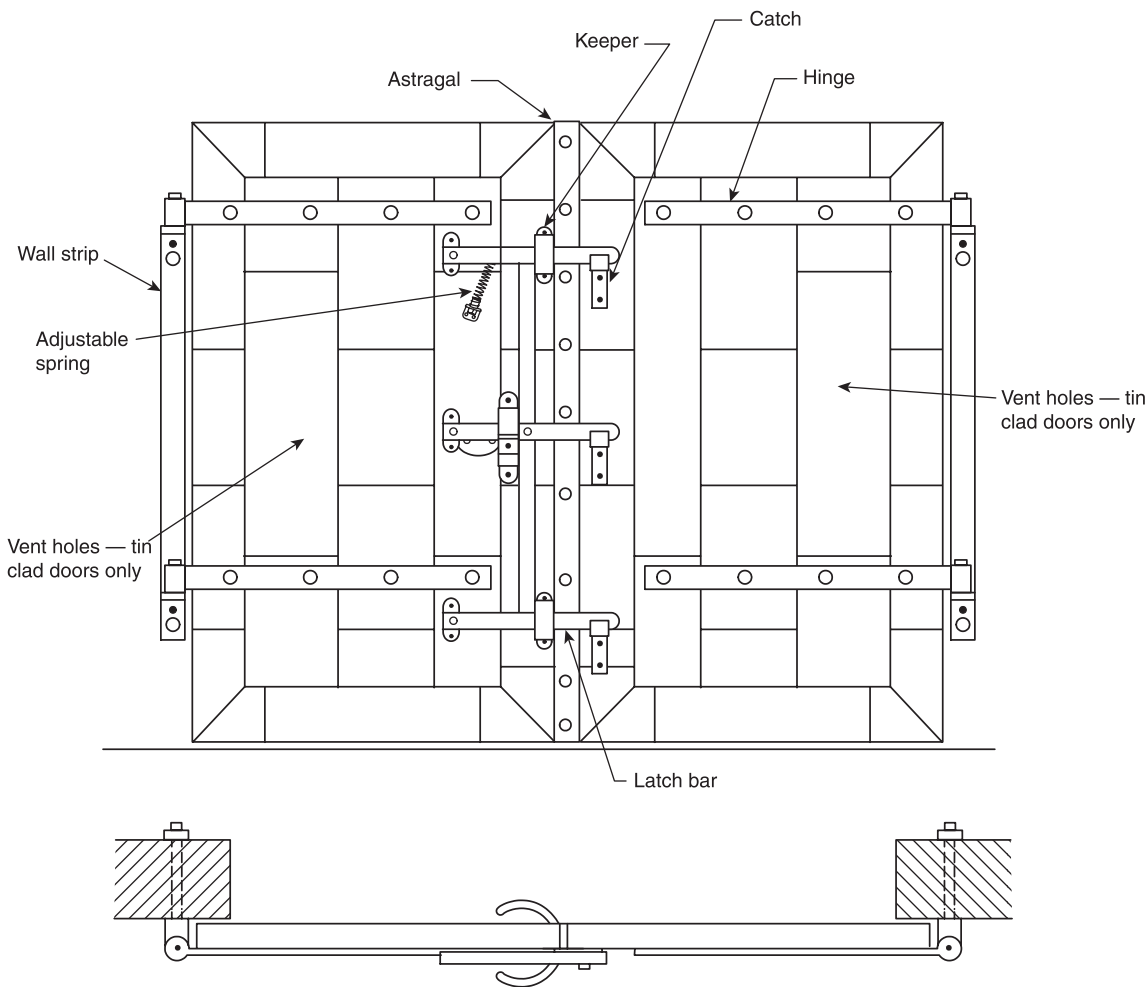
N FIGURE A.7.1(c) Fire Door Hardware (Doors Swinging in Pairs — Lap Mounted).
