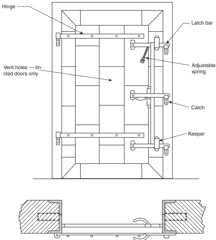
N FIGURE A.7.1(a) Fire Door Hardware (Single Swinging Door — Flush Mounted).
