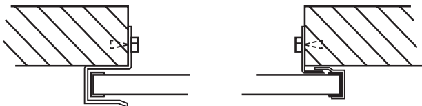
FIGURE A.4.6.4(f) Binder Arrangements.
