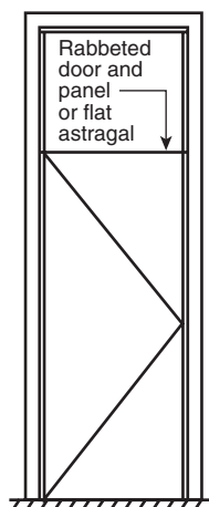
FIGURE A.3.3.53(a) Transom Panel Frame Without Transom Bar.
