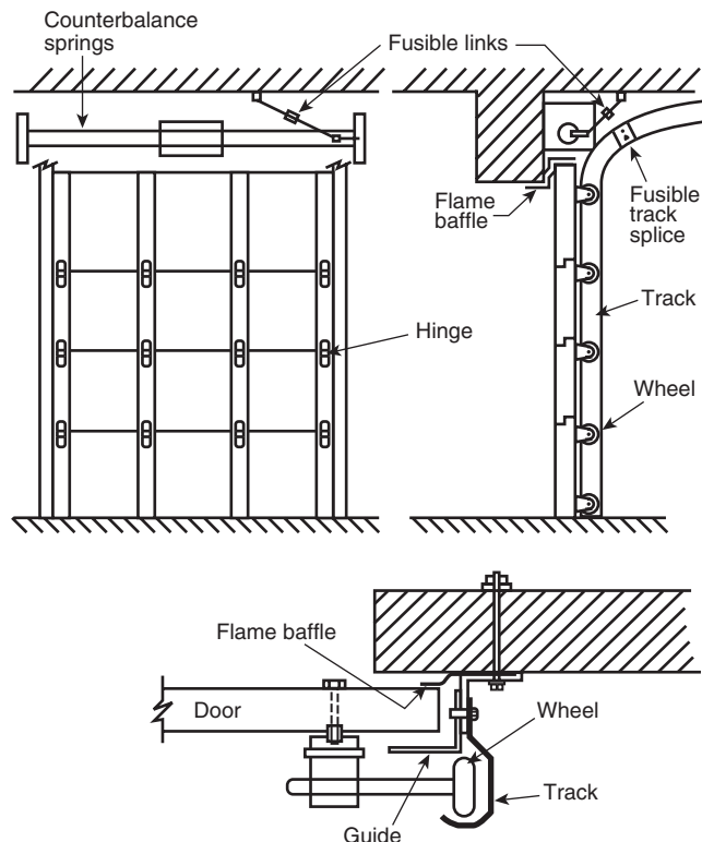
FIGURE A.4.7.5(j) Vertically Sliding, Steel-Sectional Overhead Door.
