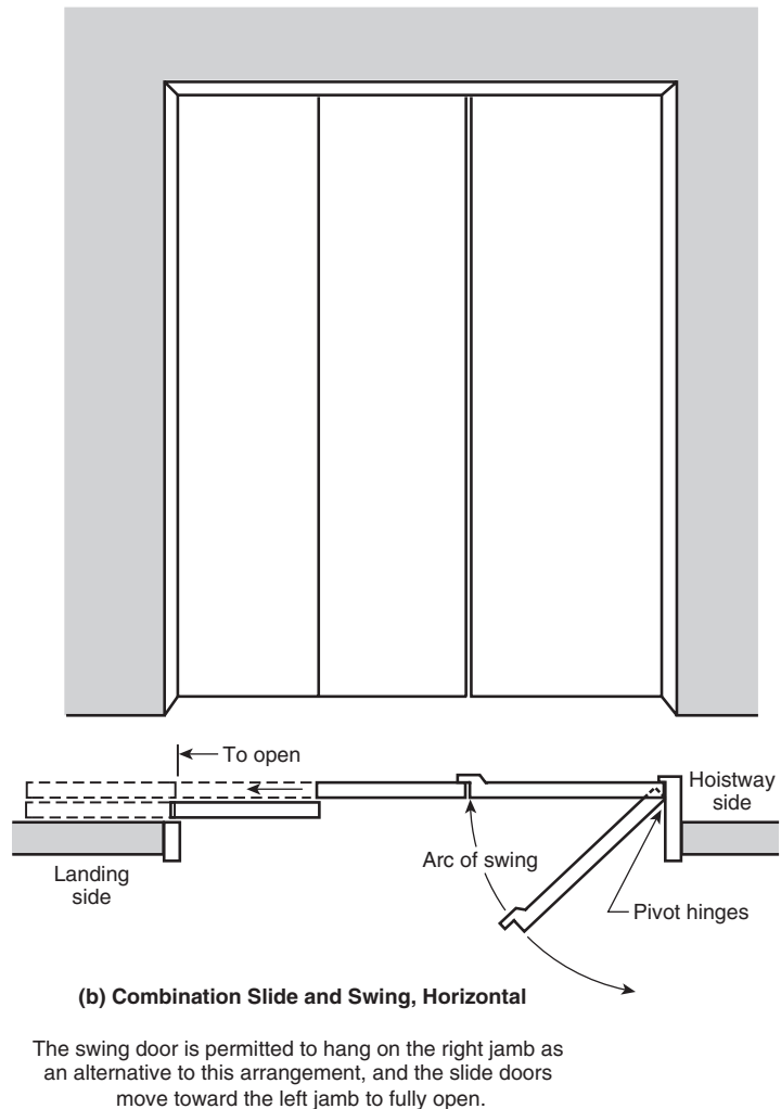
FIGURE A.14.2.1.3 Horizontal Swinging and Horizontal Combination Sliding and Swinging Doors. (Courtesy of ASME A17.1, Handbook on Safety Code for Elevators and Escalators .)
