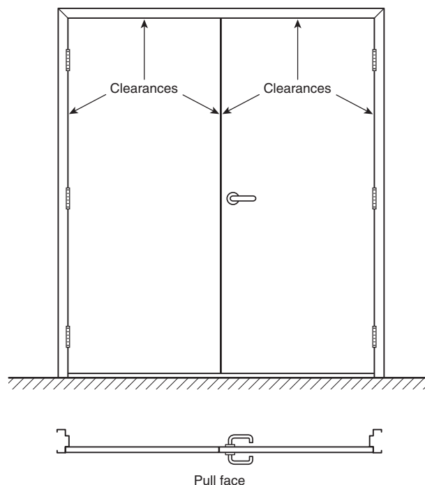
FIGURE A.6.3.1.7 Pull Face of a Swinging Pair of Doors.
