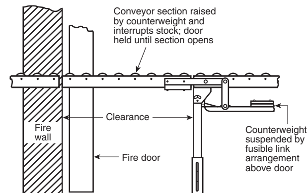
FIGURE B.4(d) Counterweight-Hinged Section of Roller Conveyor.
