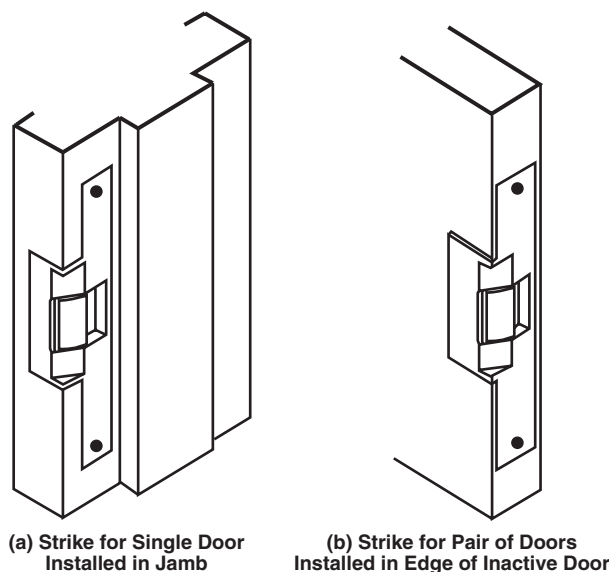
FIGURE A.6.4.4.11 Typical “Electric Strike” for Single Swing and Pair of Doors Where Permitted by Individual Listings.
