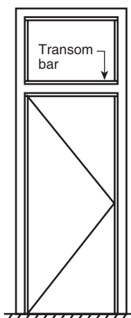
FIGURE A.3.3.53(b) Transom Panel Frame with Transom Bar.
