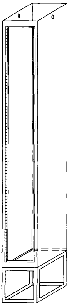
Figure 5-2(a) Orthographic view of flame testing apparatus.
