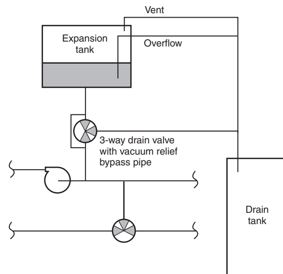
FIGURE A.8.3.2.5.3(b) Expansion Tank Isolation Using a Three-Way Valve.
