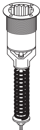
FIGURE A.3.3.74.5.2 Flush-Type Full Internal Pressure Relief Valve.
