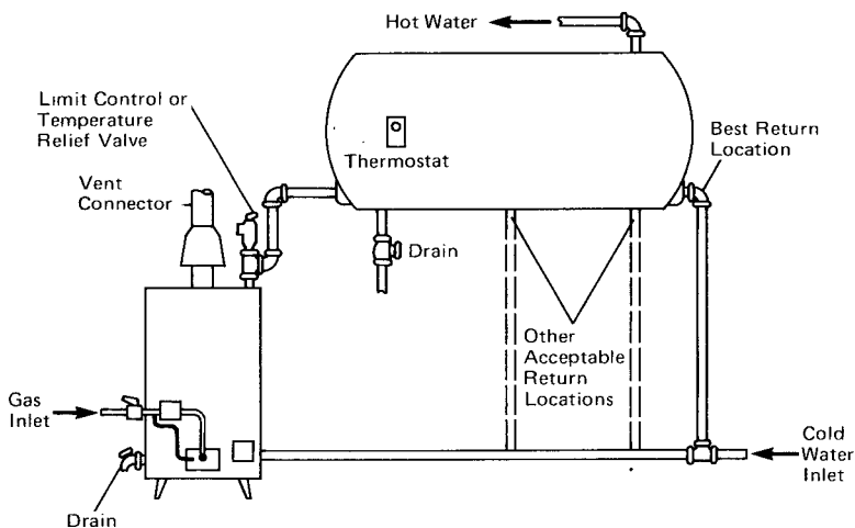
Figure 11. Typical Gravity Circulating Tank Type Installation.
