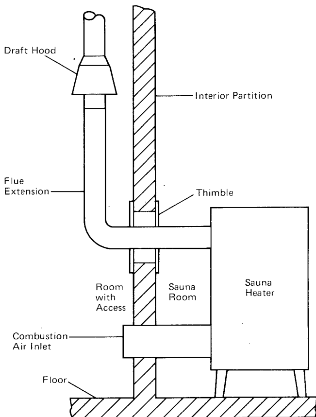
Figure 9. Typical Sauna Heater Installation.
