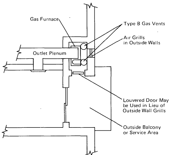
Figure 14. Plan View of Practical Separation Method for Multistory Gas Venting.
