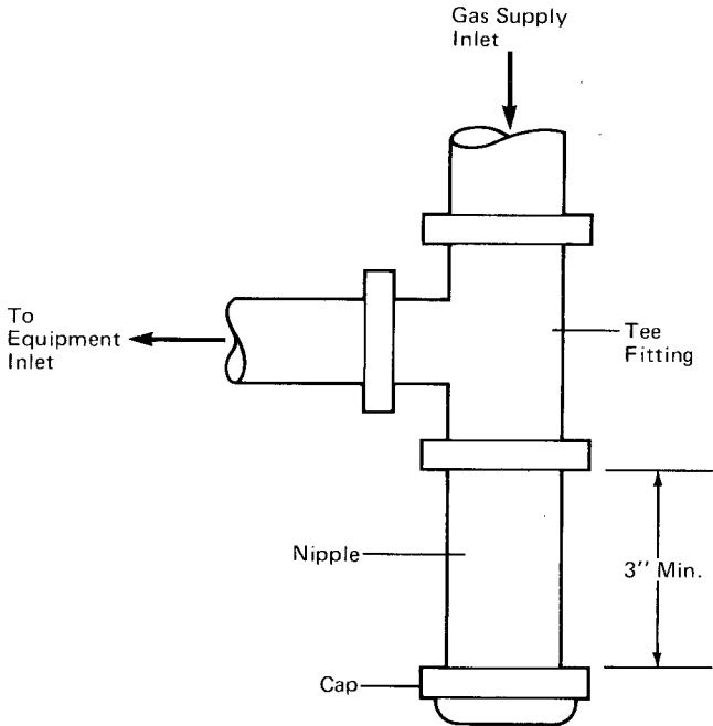
Figure 5. Method of Installing a Tee Fitting Sediment Trap.
