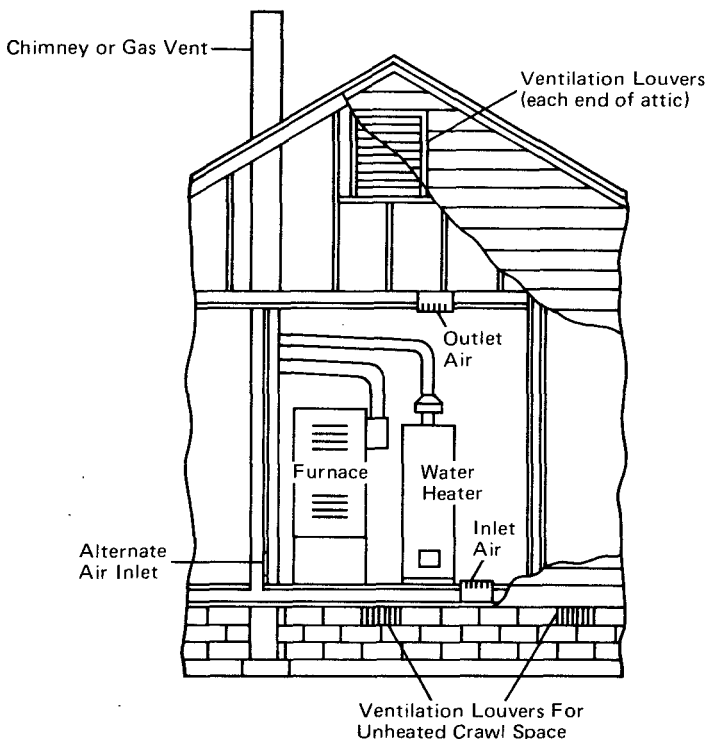
Figure 2. Equipment Located in Confined Spaces; All Air from Outdoors — Inlet Air from Ventilated Crawl Space and Outlet Air to Ventilated Attic. See 5.3.3(b).
