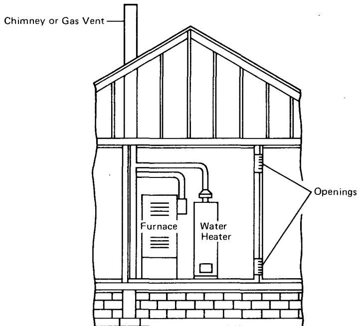
Figure 1. Equipment Located in Confined Spaces; All Air from Inside the Building. See 5.3.3(a).
