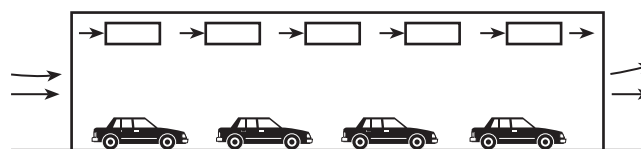
FIGURE I.2.1(c) Longitudinal Ventilation System with Jet Fans.
