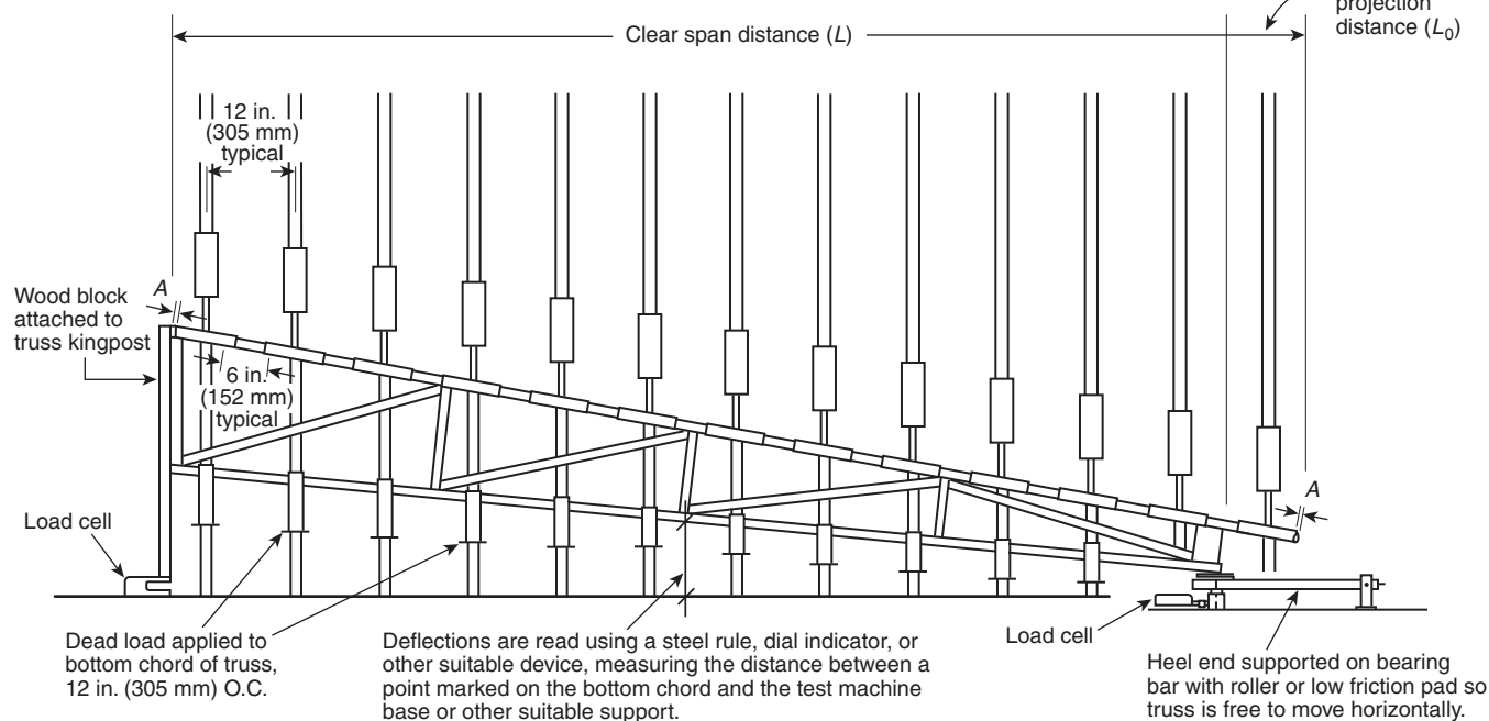
FIGURE 7.2.2.1 Test Fixture for Testing Trusses Singly.
