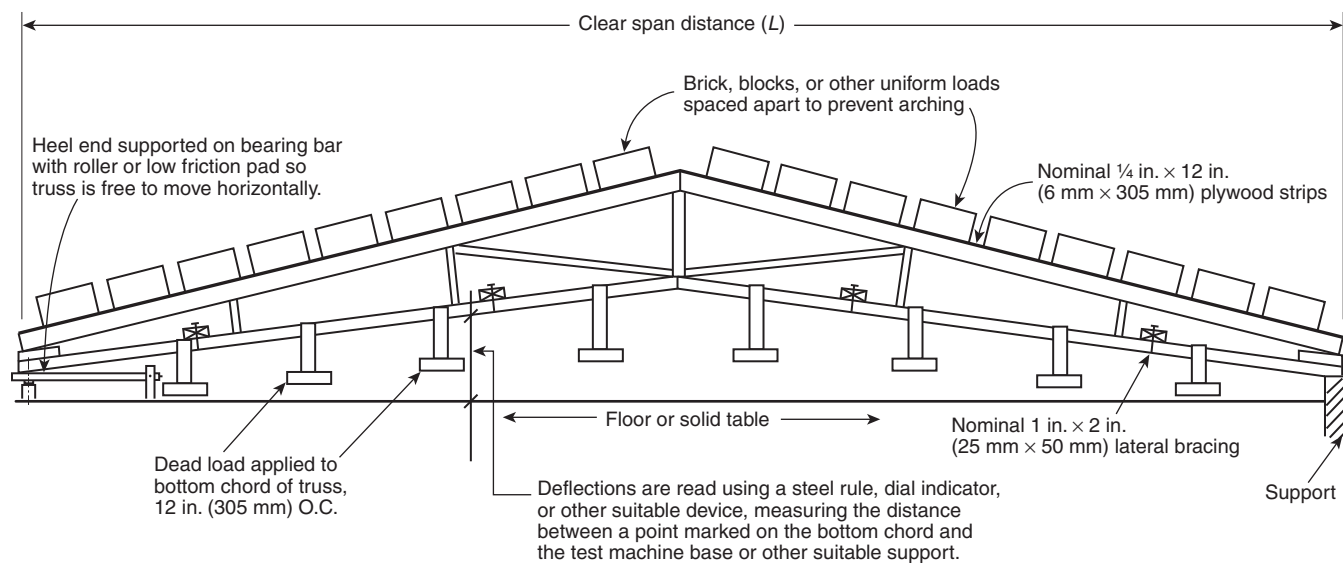
FIGURE 7.2.2.2 Test Setup for Roof Trusses Tested in Groups of Two or More.
