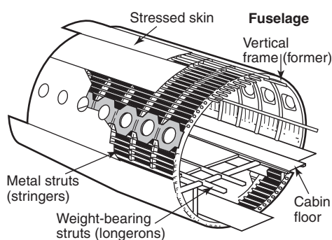
FIGURE 8.1.2 Fuselage Components.
