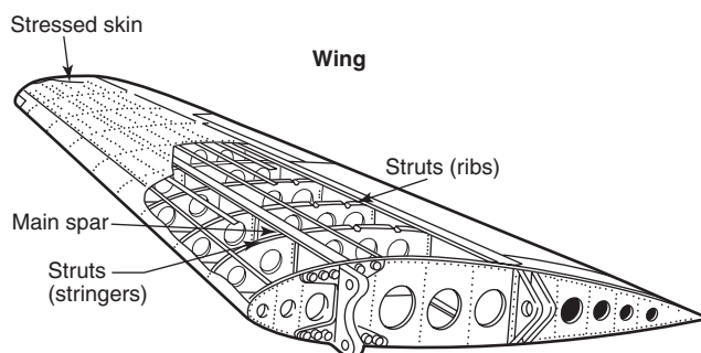
FIGURE 8.1.3 Wing Components.
